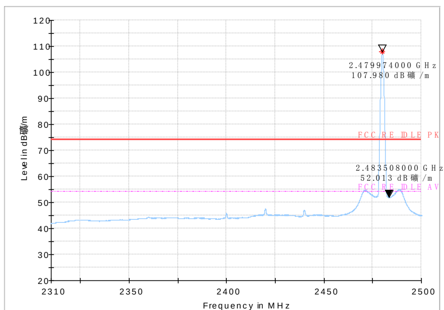
Fig.25 Bandedge:ch39
