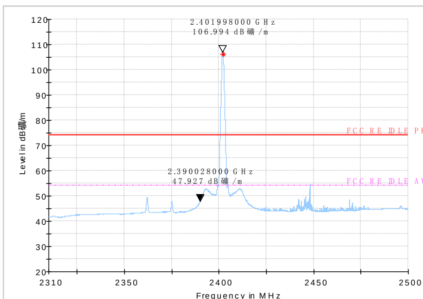
Fig.21 Bandedge:ch0
