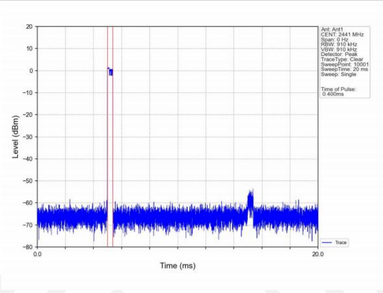
Dwell_Time_(Hopping)_NVNT_ANT1_2-DH1_2441_Accumulated
