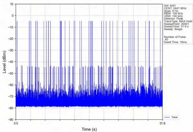
Dwell_Time_(Hopping)_NVNT_ANT1_3-DH1_2441_Accumulated
