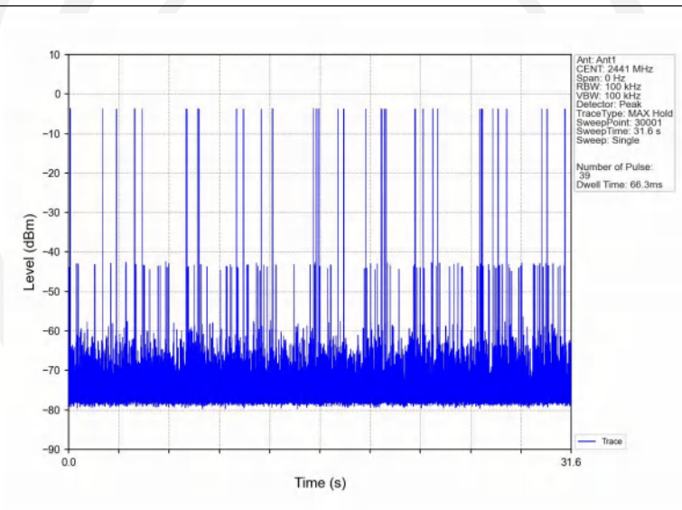
Dwell_Time_(Hopping)_NVNT_ANT1_3-DH3_2441_Accumulated
