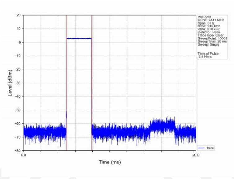
Dwell_Time_(Hopping)_NVNT_ANT1_DH5_2441_Accumulated
