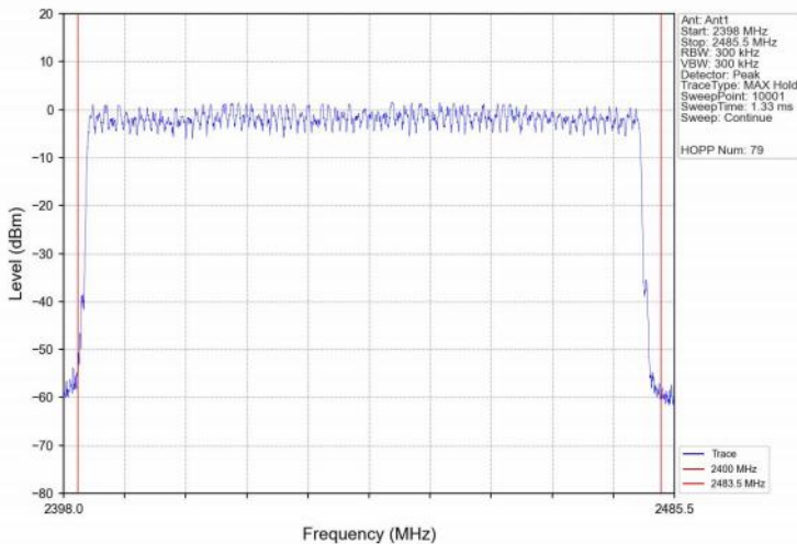
Number_of_Hopping_Channel_(Hopping)_NVNT_ANT1_2DH5_Hopping
