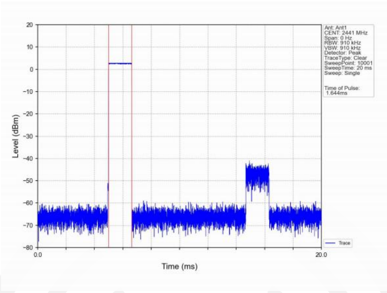
Dwell_Time_(Hopping)_NVNT_ANT1_DH3_2441_Accumulated
