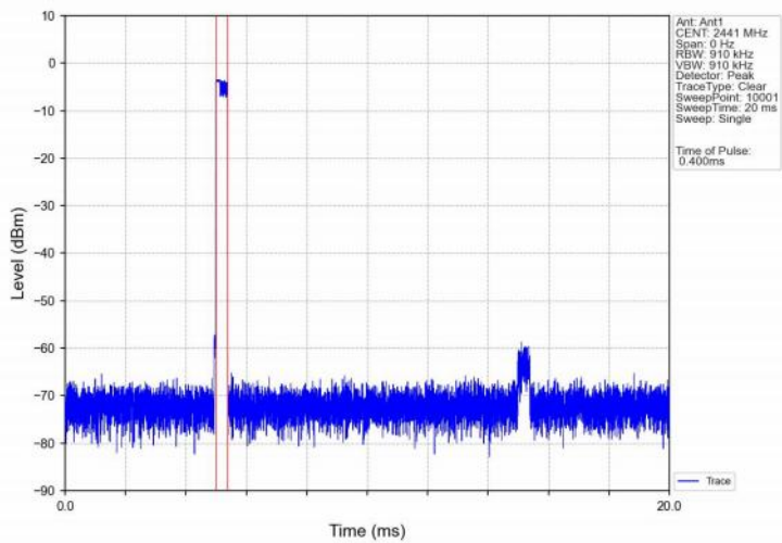
Dwell_Time_(Hopping)_NVNT_ANT1_3-DH1_2441_Accumulated
