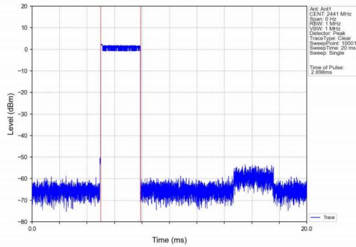
Dwell_Time_(Hopping)_NVNT_ANT1_2-DH5_2441_Accumulated
