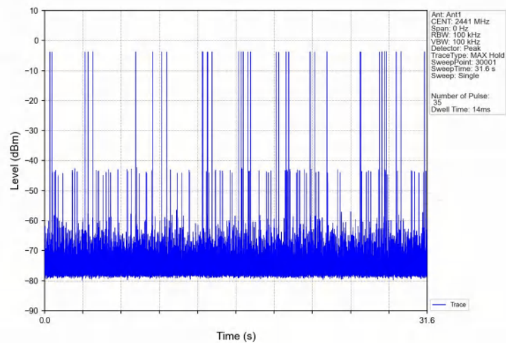
Dwell_Time_(Hopping)_NVNT_ANT1_3-DH1_2441_Accumulated
