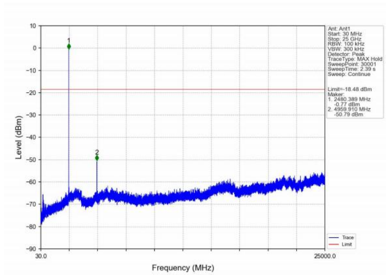
GFSK_DH5_HCH_2480MHz_Ant1_NTNV
