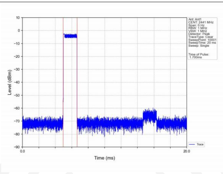
Dwell_Time_(Hopping)_NVNT_ANT1_3-DH3_2441_Accumulated
