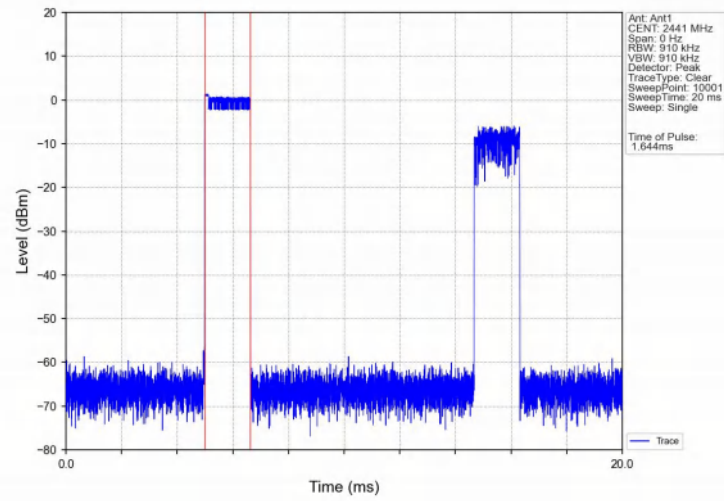
Dwell_Time_(Hopping)_NVNT_ANT1_2-DH3_2441_Accumulated
