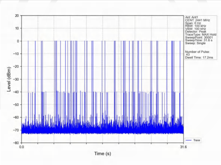
Dwell_Time_(Hopping)_NVNT_ANT1_2-DH1_2441_Accumulated
