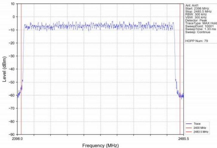
Number_of_Hopping_Channel_(Hopping)_NVNT_ANT1_3DH5_Hopping
