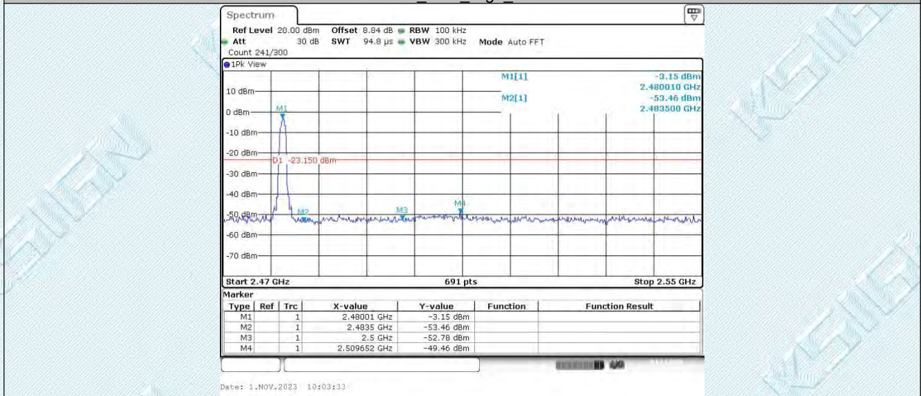
3DH5_Ant1_High_2480
