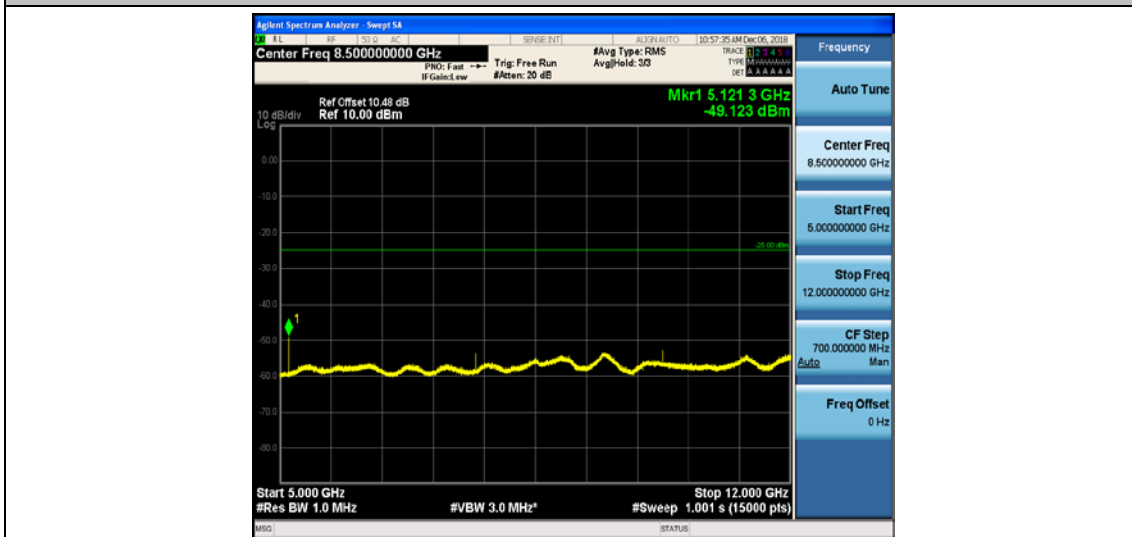
Band7_10MHz_QPSK_21400_1RB#0
