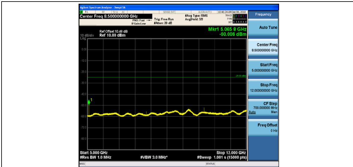
Band7_5MHz_QPSK_21100_1RB#0
