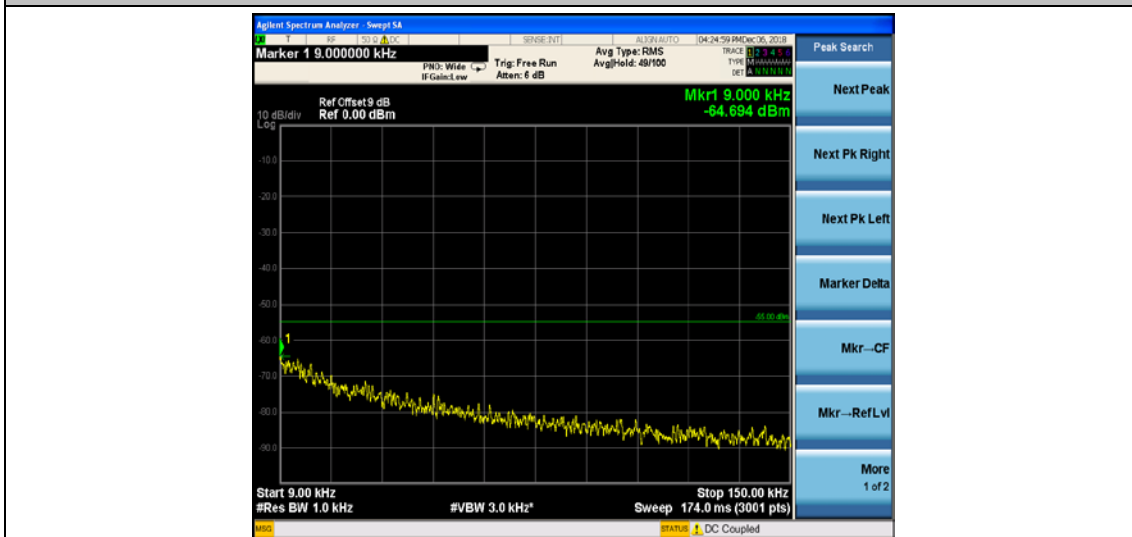
Band7_10MHz_16QAM_20800_1RB#0
