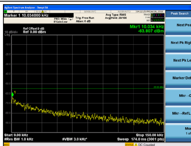
Band7_5MHz_QPSK_21100_1RB#0
