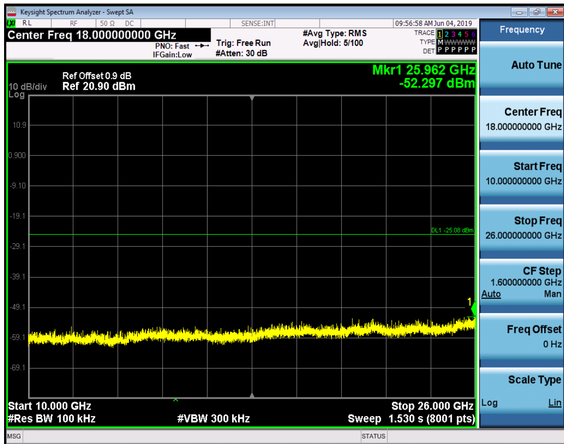
RF Conducted Spurious Emissions_DH5_2480
