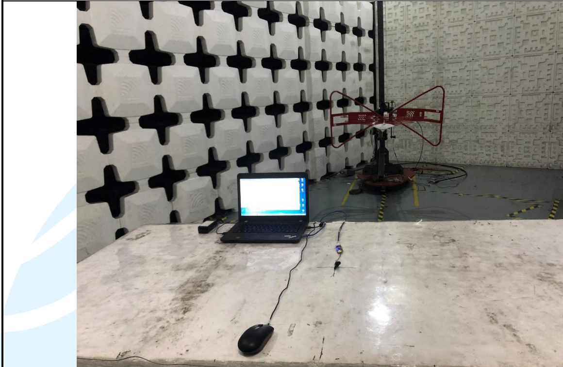
Radiated emission Test Setup (30 MHz~1 GHz) _Left earbud
