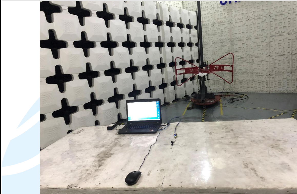
Radiated emission Test Setup (30 MHz~1 GHz) _Right earbud
