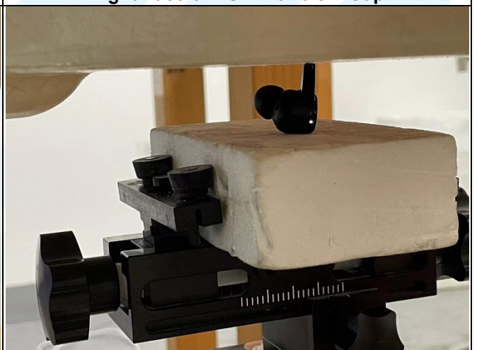
Bottom Face of EUT with 0 cm Gap
