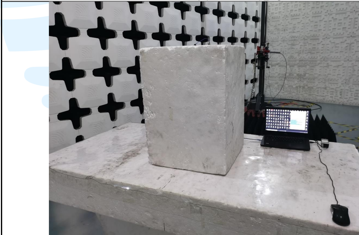
Radiated emission Test Setup (Above 1 GHz) _Right earbuds
