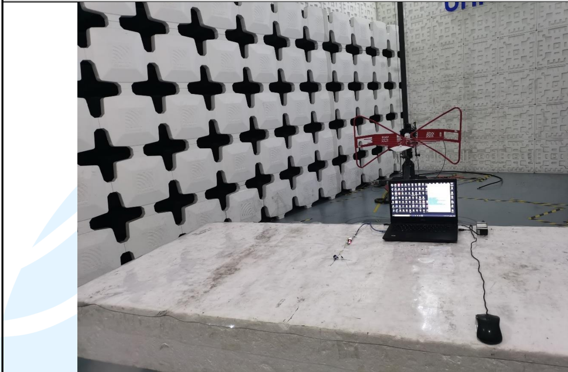
Radiated emission Test Setup (30 MHz~1 GHz) _Right earbuds
