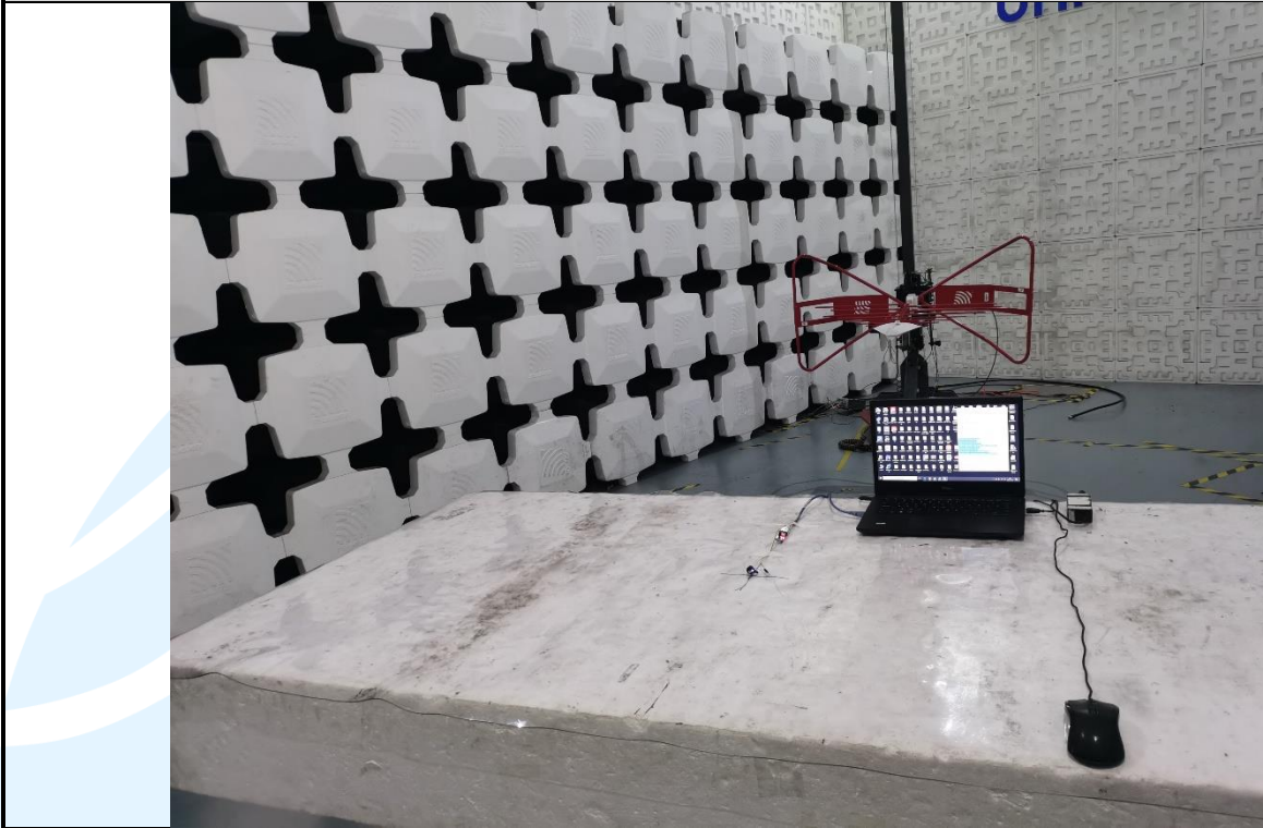
Radiated emission Test Setup (30 MHz~1 GHz) _Left earbuds
