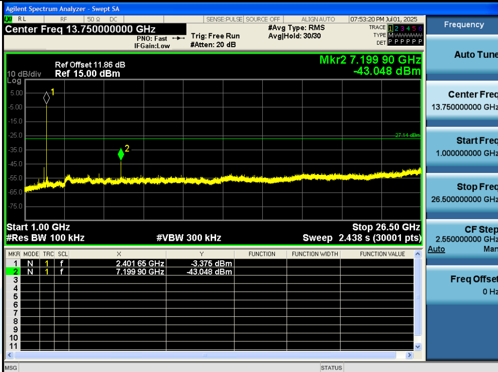
2DH5-Ant1-2402-1000~26500-PASS
