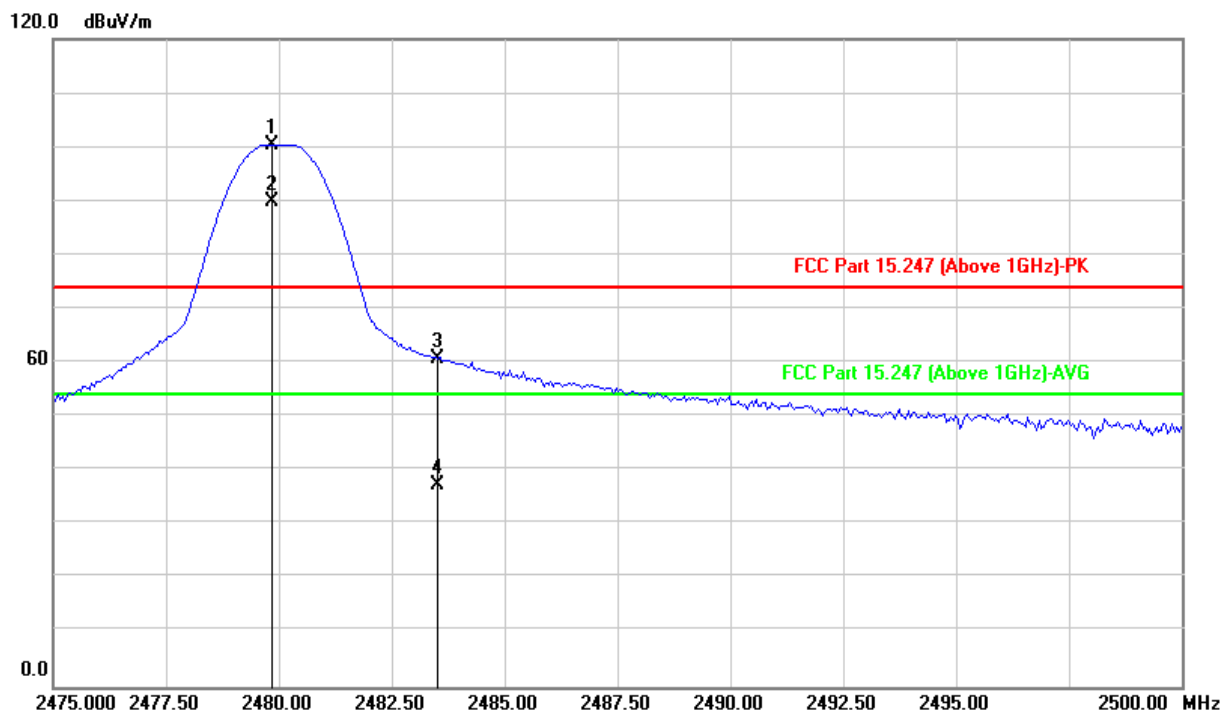
Antennal Polarity& Test Distance: Horizontal at 3 M
