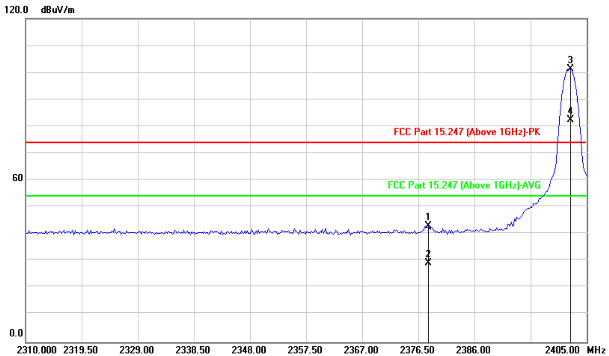
Antenna Polarity & Test Distance: Horizontal at 3 m
