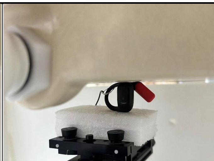
Test Position 6 (EUT with 0 cm Gap)
