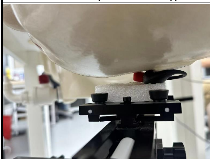
Left Cheek (EUT with 0 cm Gap)
