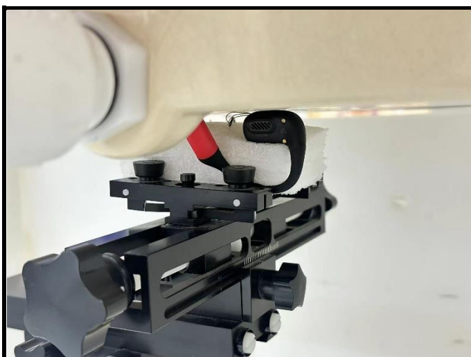
Test Position 3 (EUT with 0 cm Gap)
