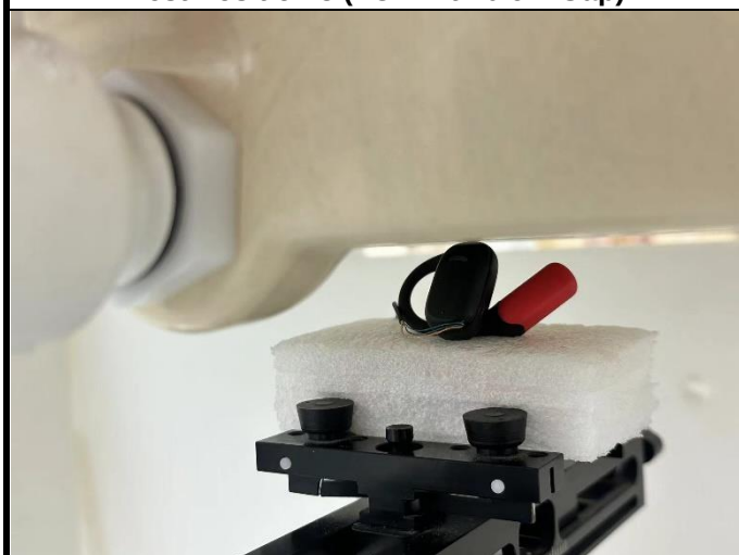
Test Position 5 (EUT with 0 cm Gap)
