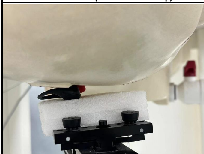
Right Cheek (EUT with 0 cm Gap)
