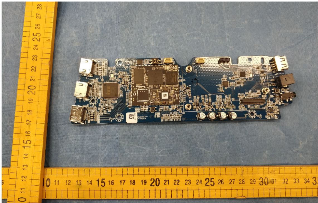
Internal View of EUT-8(sound bar)
