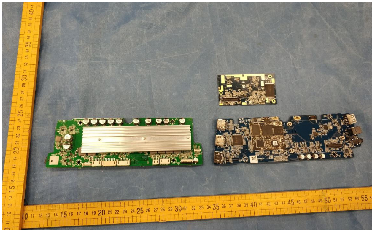
Internal View of EUT-4(sound bar)
