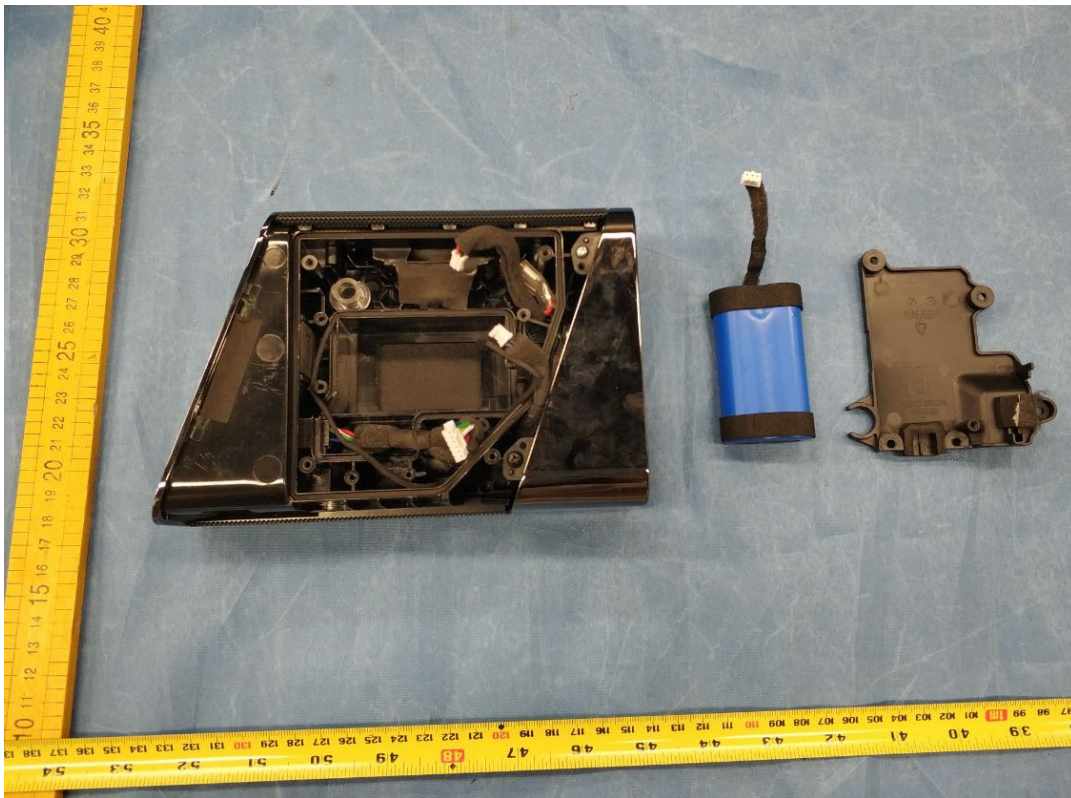
Internal View of EUT-20 surround (left)
