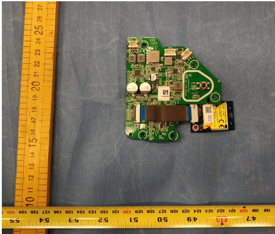
Internal View of EUT-22 surround (left)
