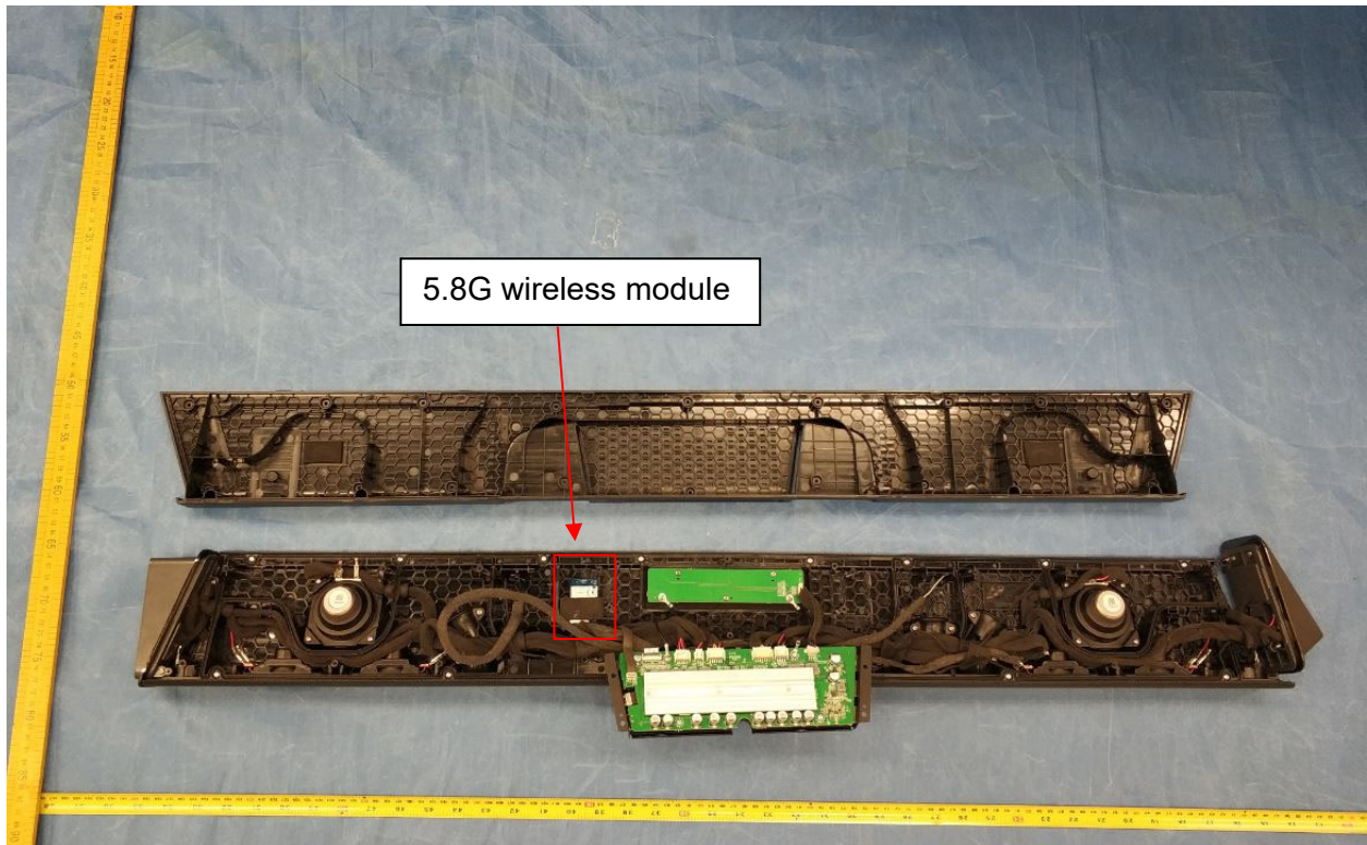
Internal View of EUT-2 (sound bar)
