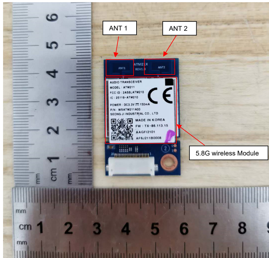
Internal View of EUT-14(sound bar)
