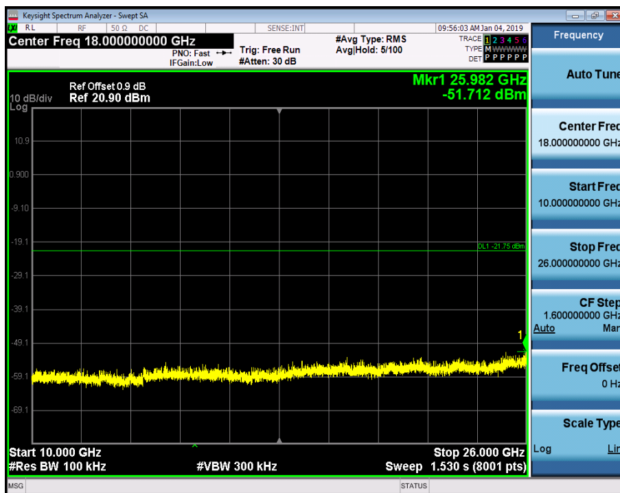
RF Conducted Spurious Emissions_3DH5_2441
