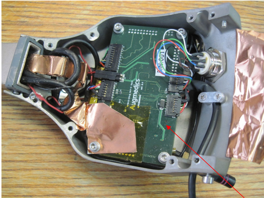
Augmedics module is on the underside of this assembly of cards as shown below
