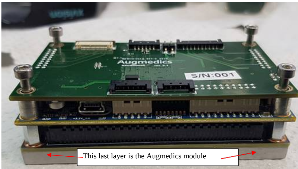
Augmedics module is on the underside of this assembly of cards as shown below
