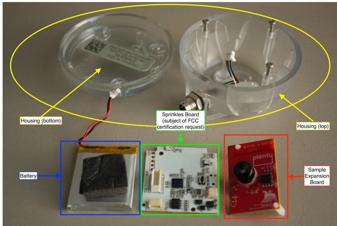
Figure 4: Disassembled Sprinkle
