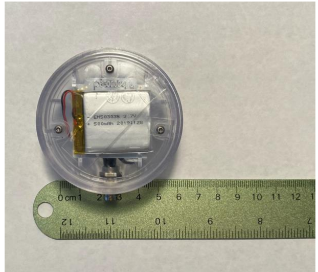
Figure 2: ASSEMBLED DEVICE, BOTTOM VIEW
