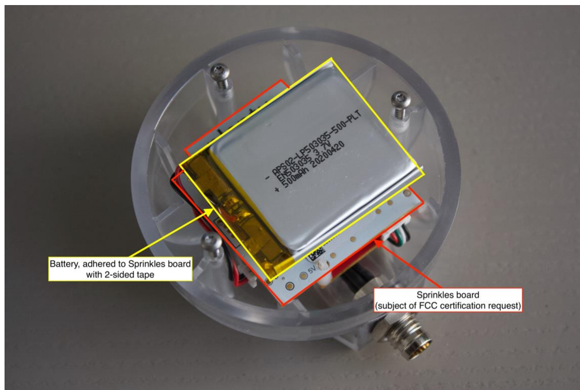
Figure 5: Partially assembled sprinkle
