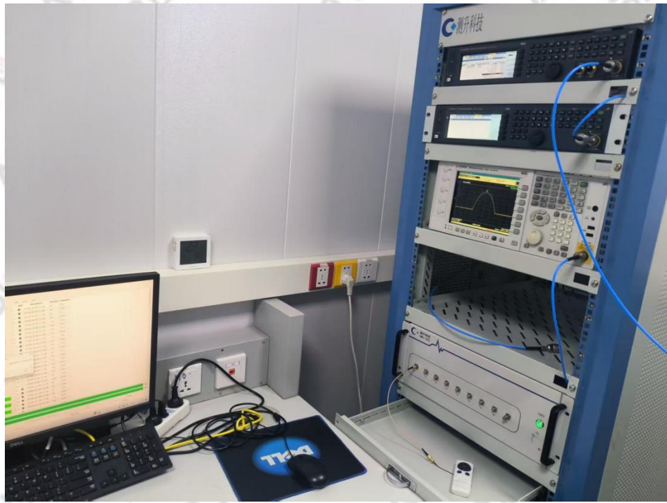
Conducted spurious emission test photos
