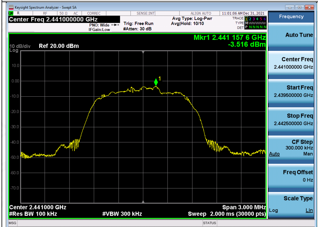
Test_Graph_EDR_ANT1_2441_3Mbps_Reference Level
