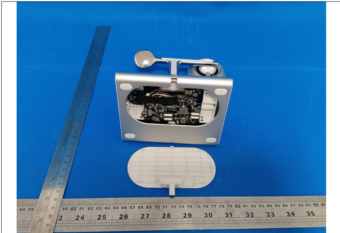
Figure 1. Internal view
