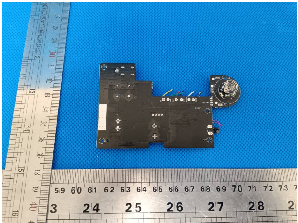
Figure 3. PCB view
