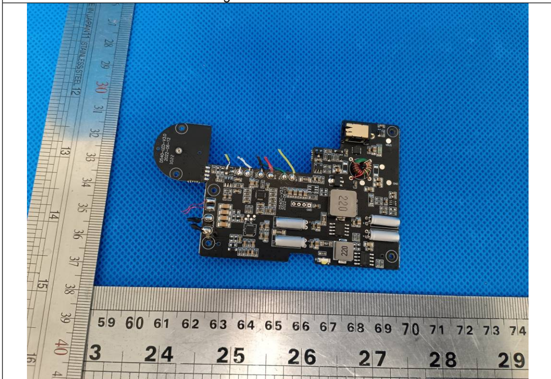
Figure 2. PCB view
