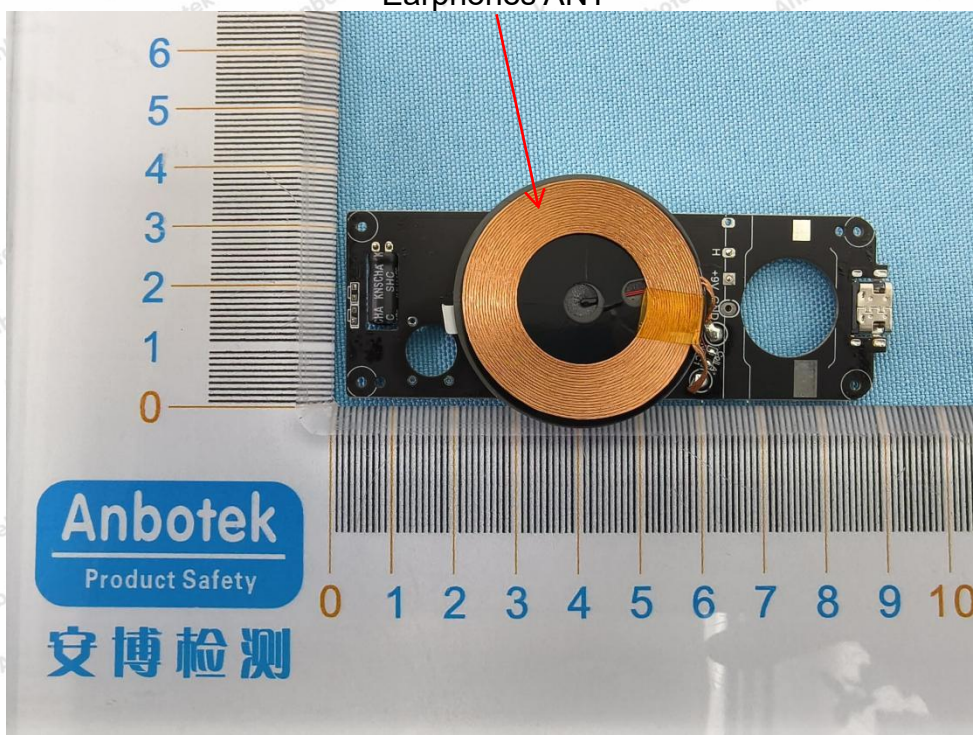
Earphones ANT
