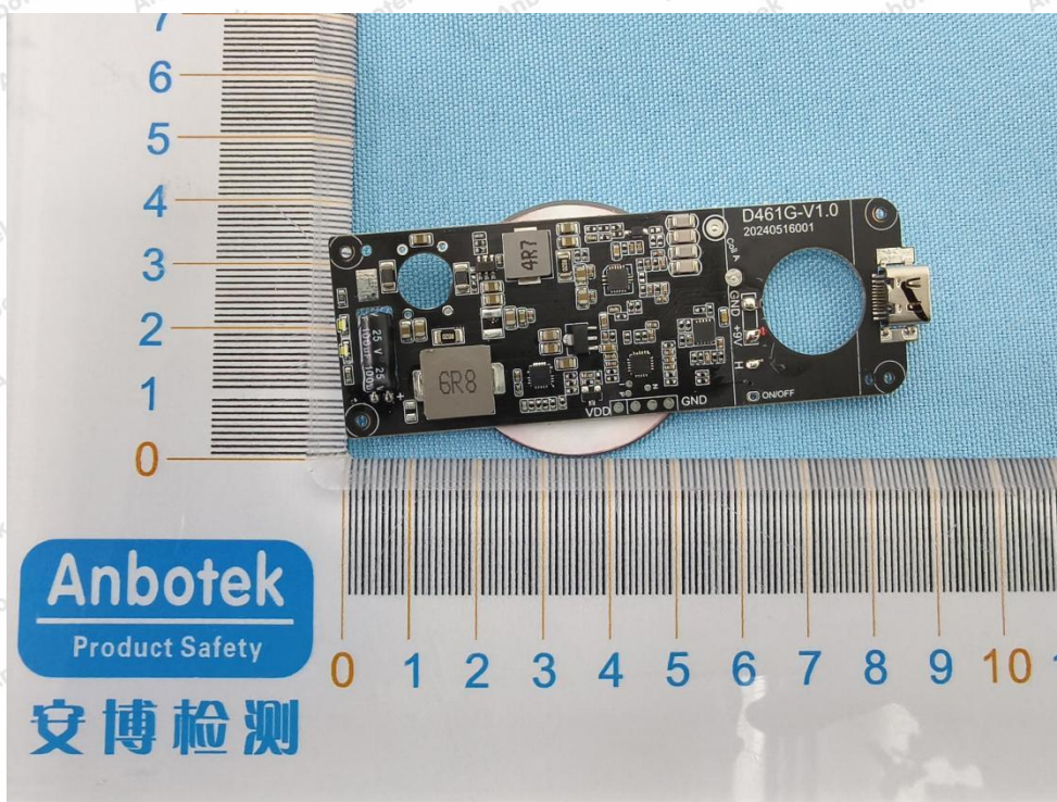
Earphones ANT
