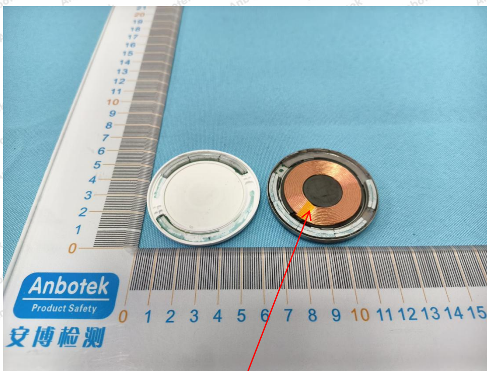
Phone ANT
