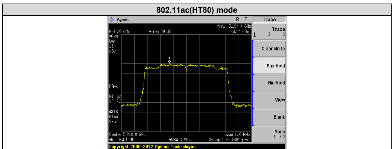
Channel 42 (5210MHz)
