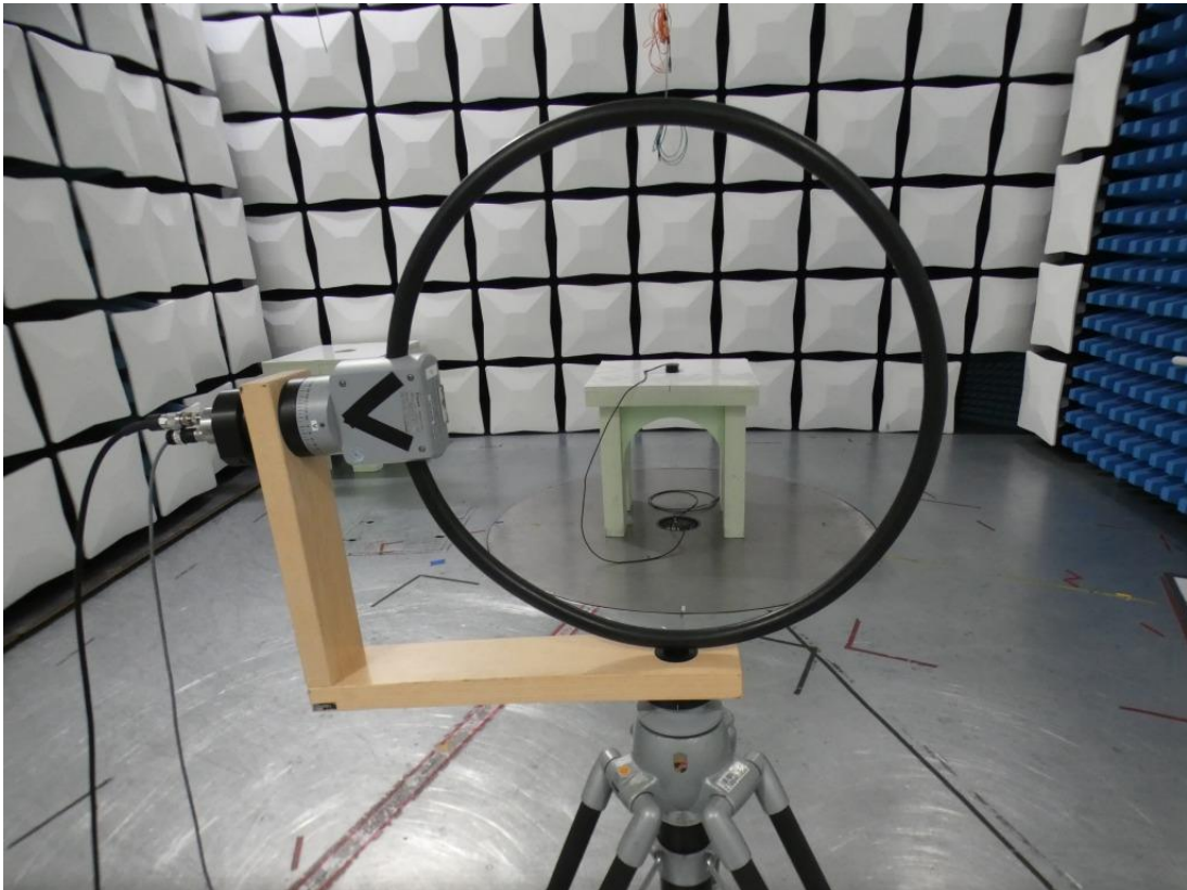
Photo 1: Test setup for radiated measurements FCC15.247, below 30 MHz
