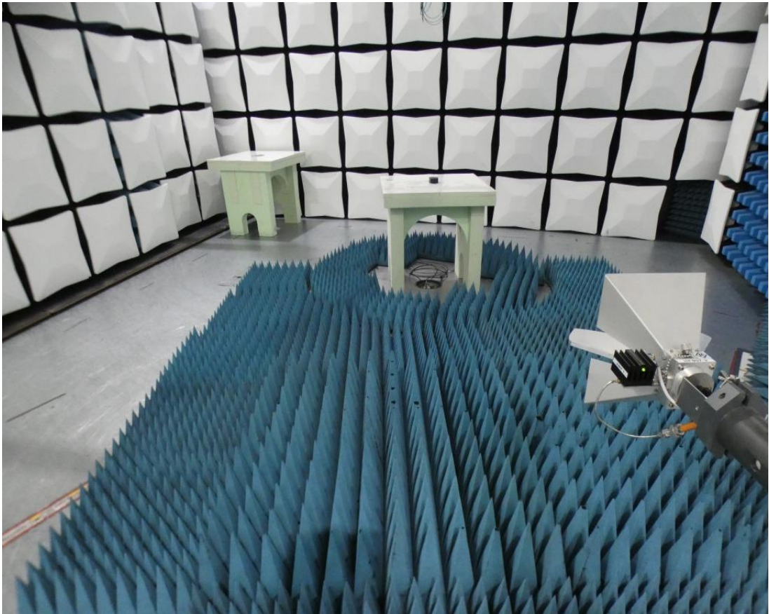
Photo 3: Test setup for radiated measurements FCC15b, above 1 GHz
