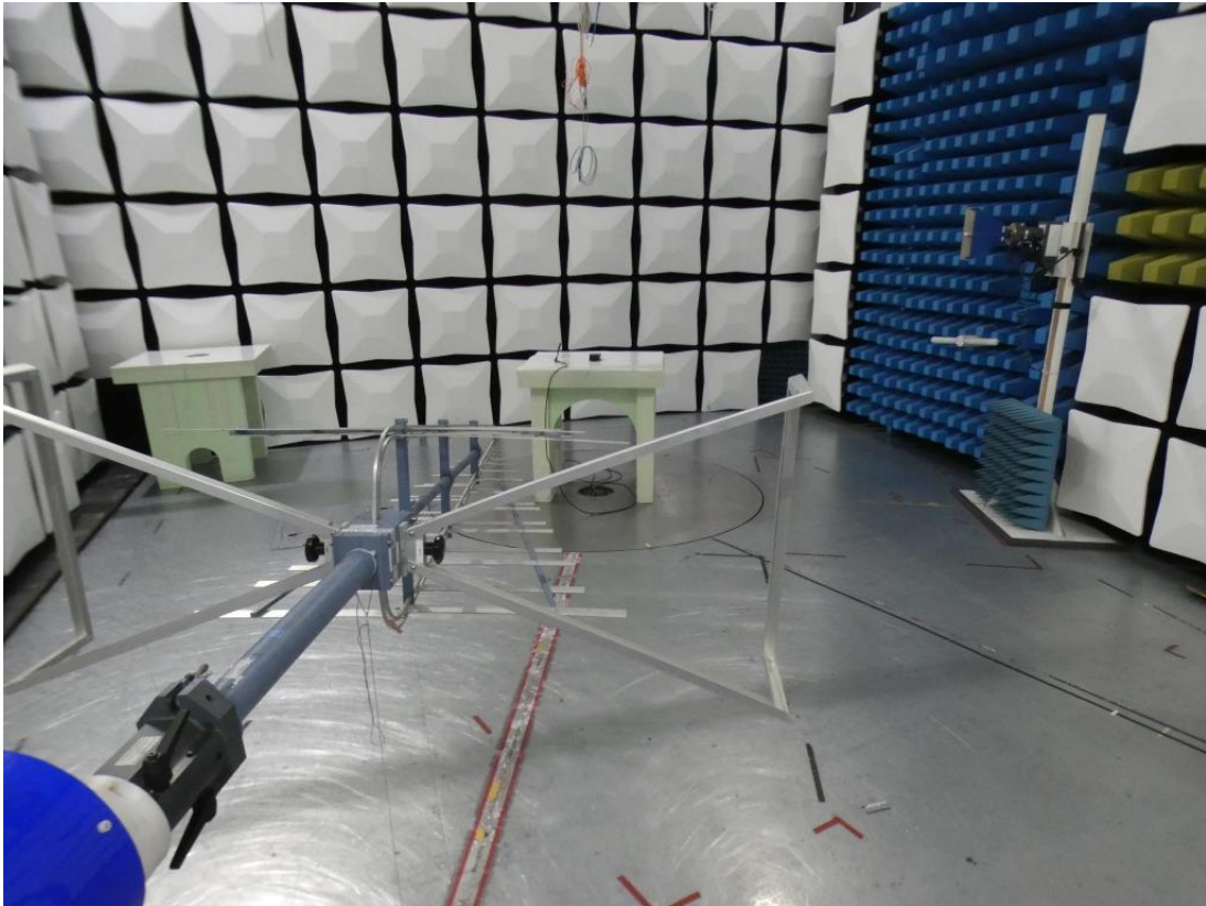
Photo 2: Test setup for radiated measurements FCC15b and FCC15.247, below 1 GHz
