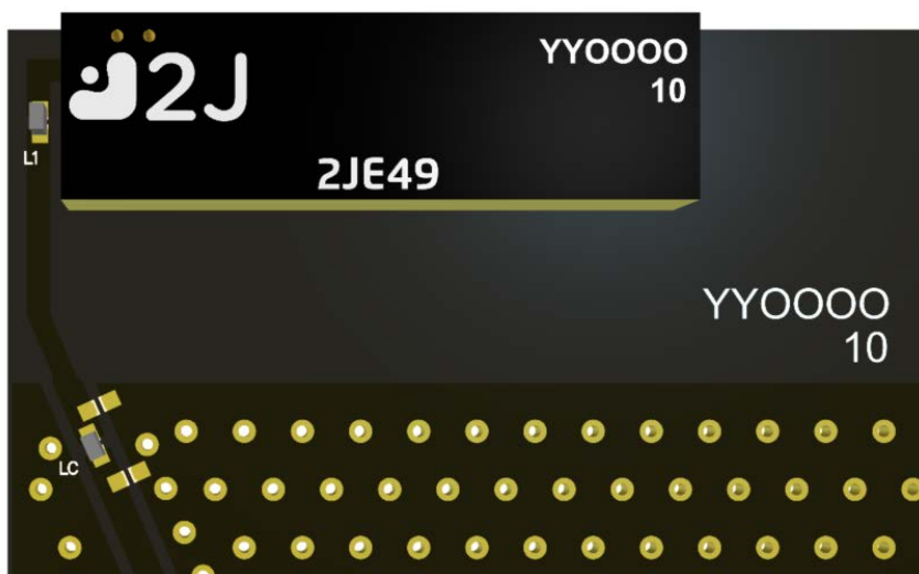
3D View of matching components and recommended values (LC = 00Ω resistor)
