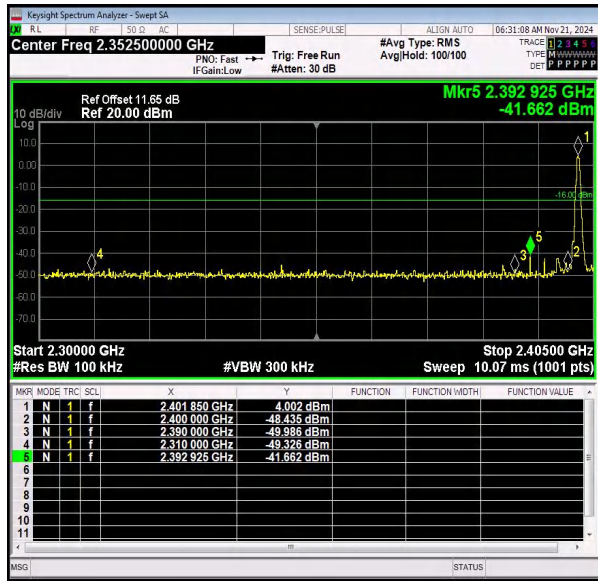
Left bandedge hopping off
