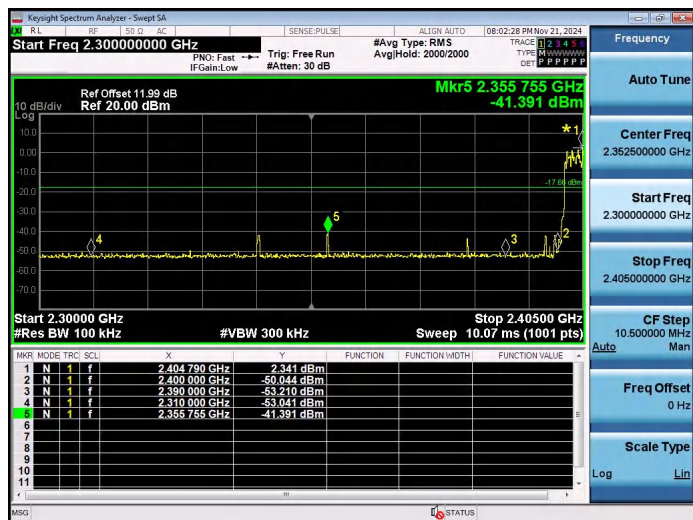
Left bandedge hopping on
