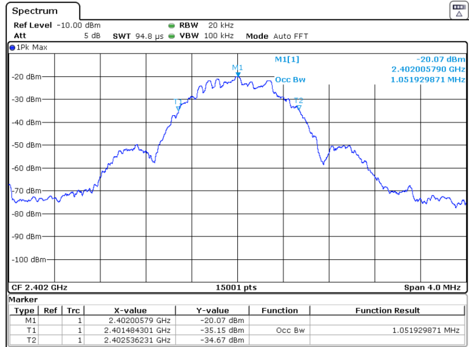
Transmission on 2402 MHz; -20°C, 24 V DC
