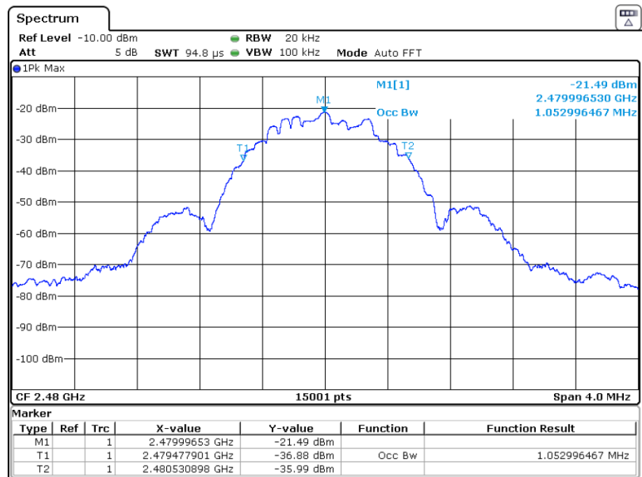
Transmission on 2480 MHz; + 50°C, 24 V DC
