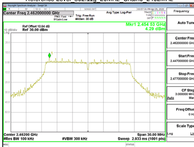
Reference Level 802.11g 20MHz Chain0 2462MHz
