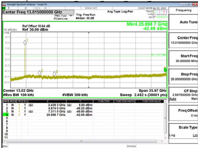
Spurious Emission 802.11b 20MHz Chain0 2437MHz
