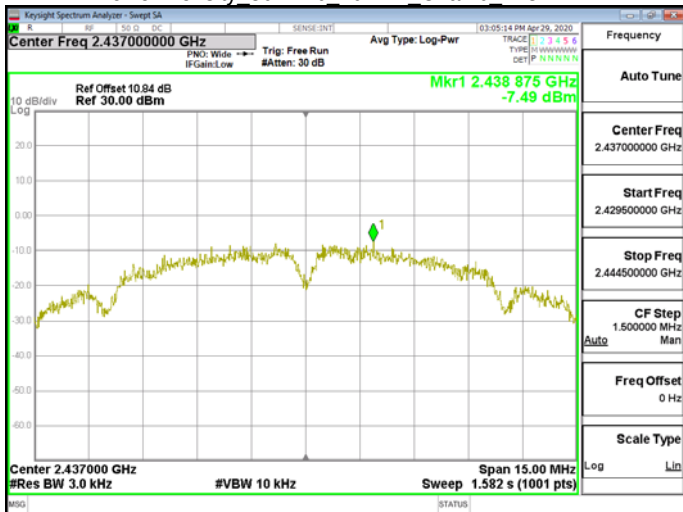
Power Density 802.11b 20MHz Chain0 2437MHz
