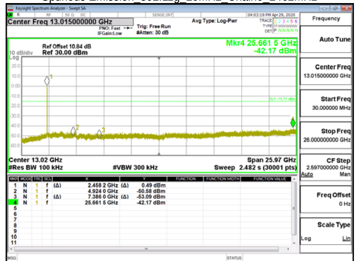
Spurious Emission 802.11g 20MHz Chain0 2462MHz
