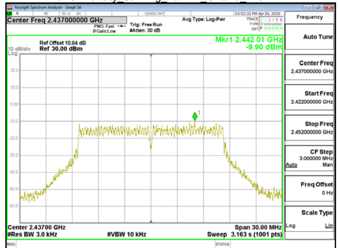
Power Density 802.11g 20MHz Chain0 2437MHz
