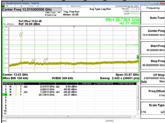
Spurious Emission 802.11b 20MHz Chain0 2412MHz
