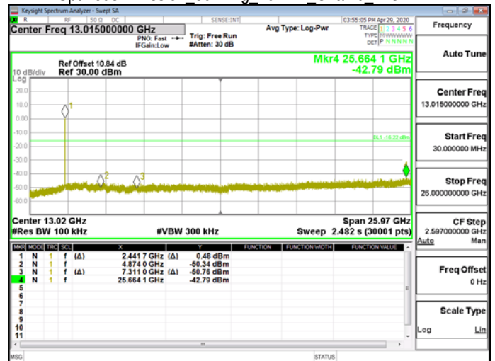
Spurious Emission 802.11g 20MHz Chain0 2437MHz
