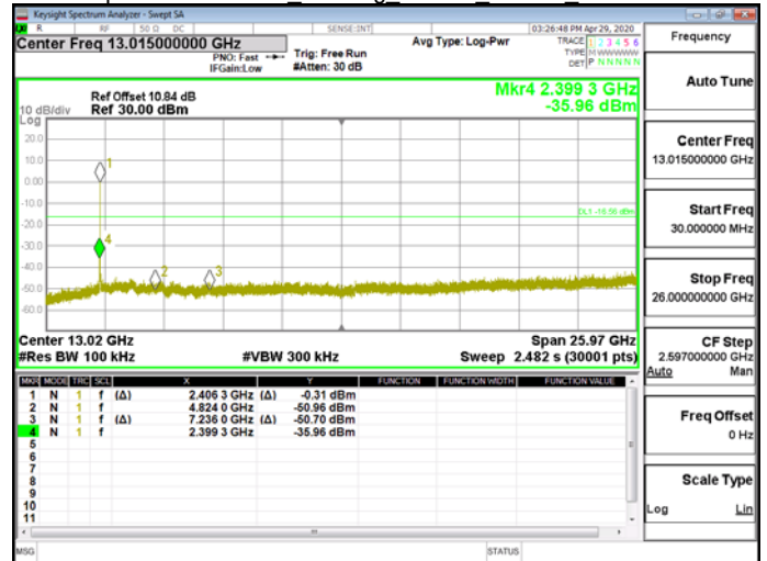
Spurious Emission 802.11g 20MHz Chain0 2412MHz
