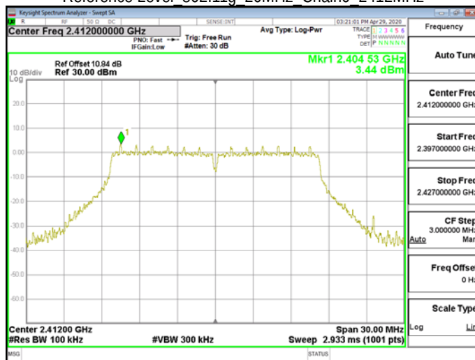
Reference Level 802.11g 20MHz Chain0 2412MHz
