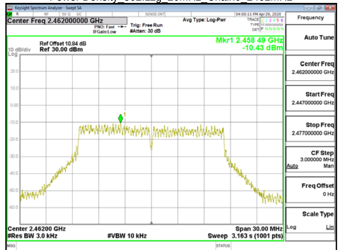
Power Density 802.11g 20MHz Chain0 2462MHz
