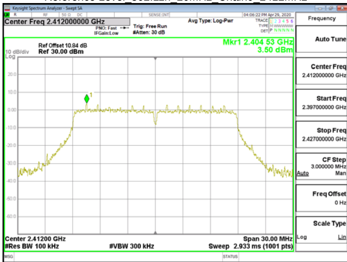
Reference Level 802.11n 20MHz Chain0 2412MHz
