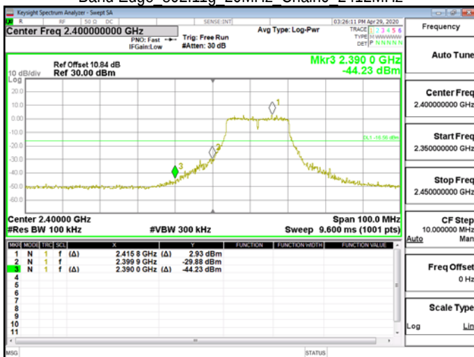
Band Edge 802.11g 20MHz Chain0 2412MHz
