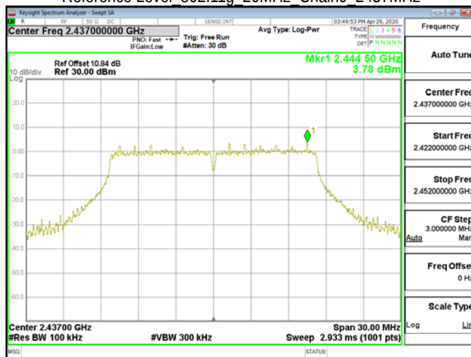
Reference Level 802.11g 20MHz Chain0 2437MHz
