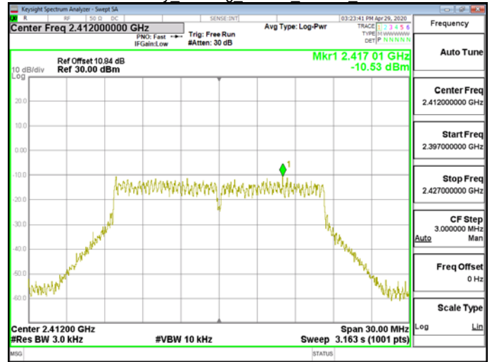
Power Density 802.11g 20MHz Chain0 2412MHz
