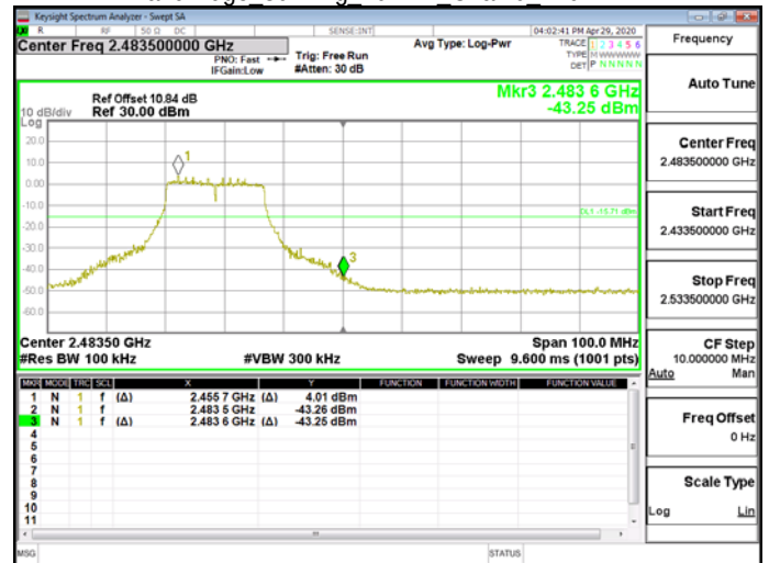
Band Edge 802.11g 20MHz Chain0 2462MHz
