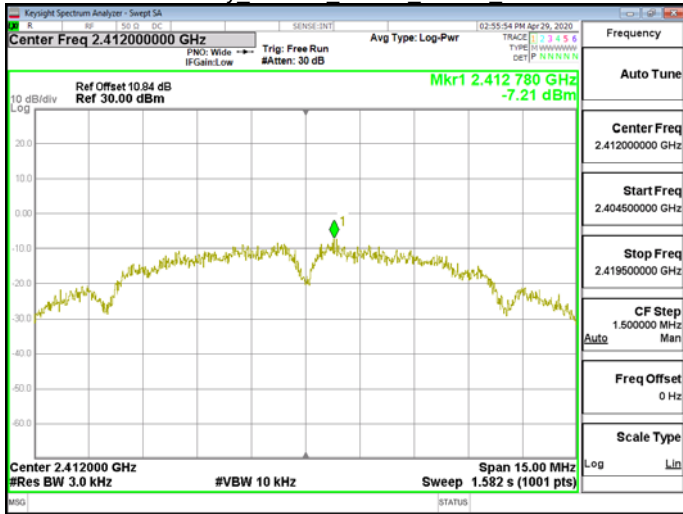
Power Density 802.11b 20MHz Chain0 2412MHz
