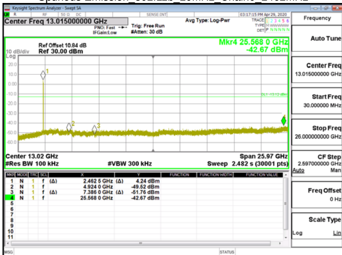
Spurious Emission 802.11b 20MHz Chain0 2462MHz
