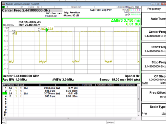
Dwell Time_8DPSK_3M_DH5_2441MHz
