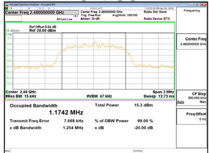
OBW 20dB_π/4QPSK_2M_2480MHz
