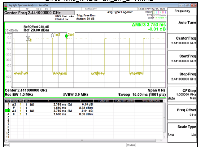
Dwell Time_π/4DQPSK_2M_2441MHz
