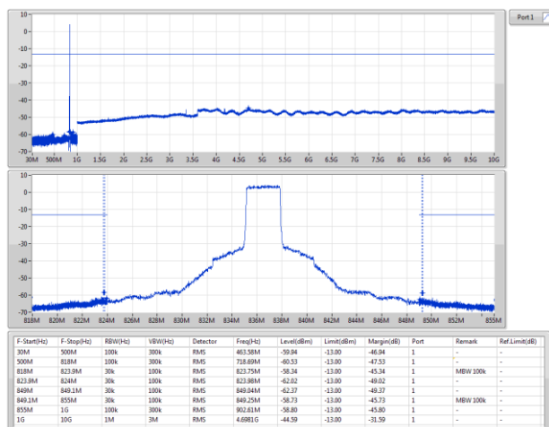
Band 5_LTE_3MHz_Nss1,QPSK_1TX 836.5MHz_QPSK_RB 15,#RB 0
