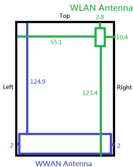
Fig.15 Front view of EUT
