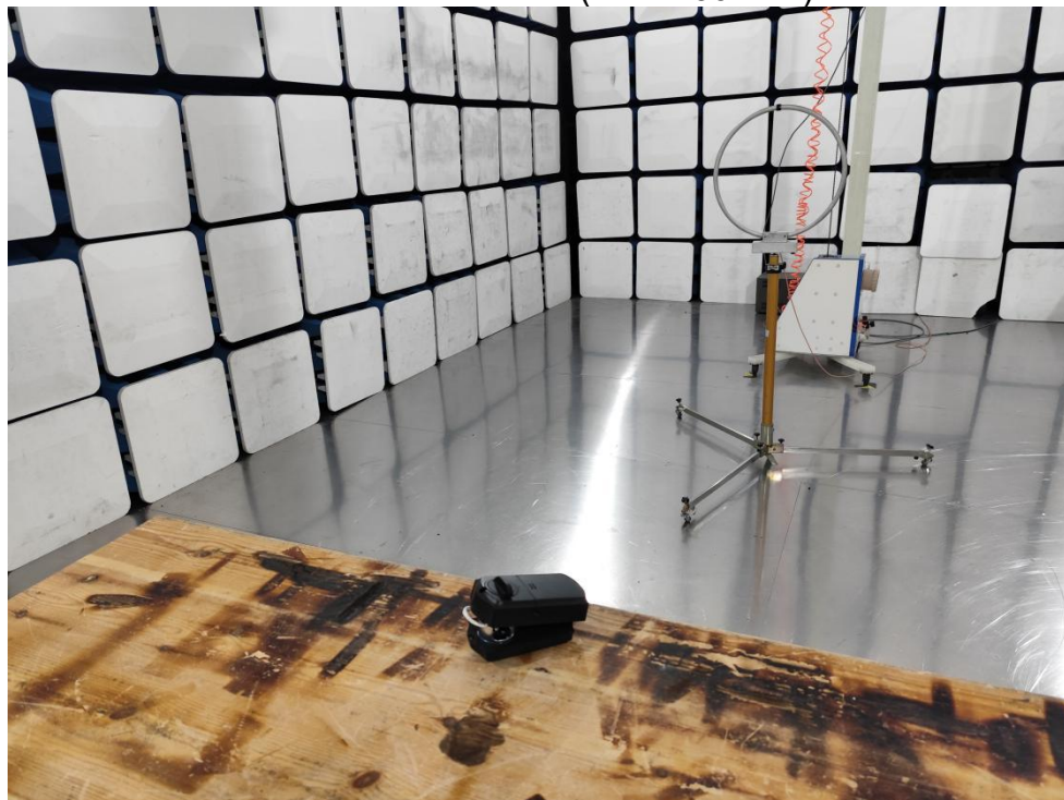
Radiation Emission (below 30MHz)
