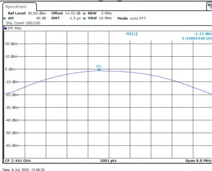
3DH5_Ant1_2441
