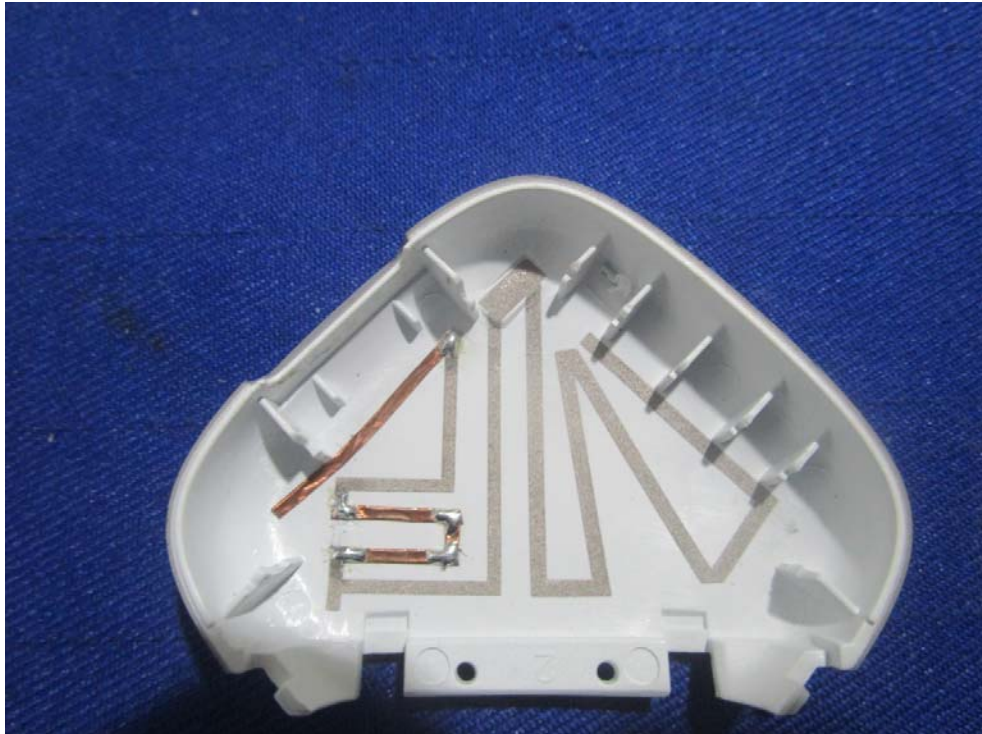
EUT – LORA Ant View
