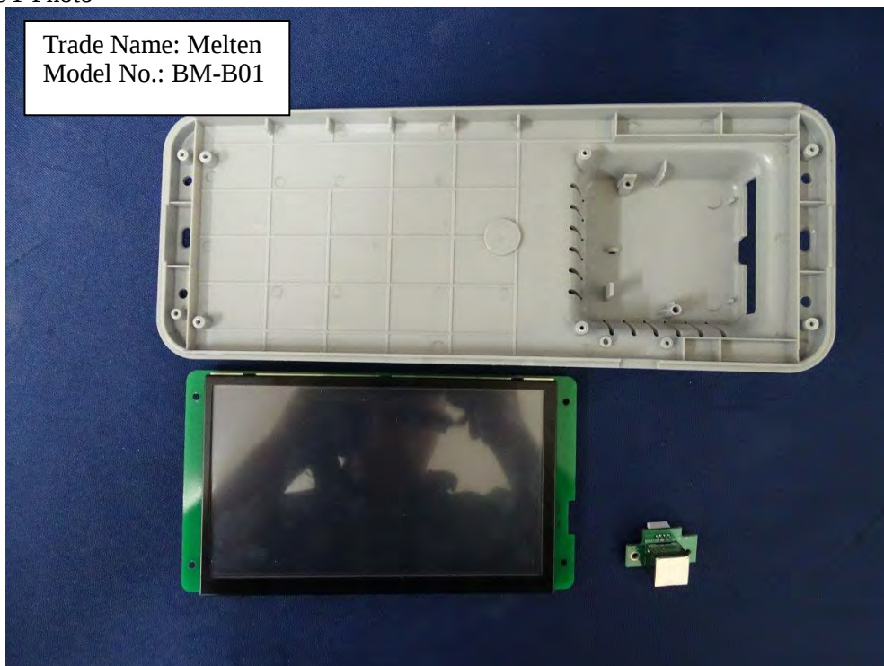
(27) EUT Photo
