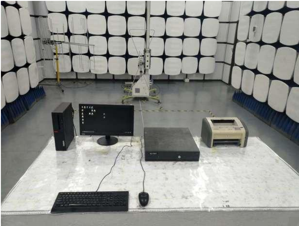
Radiated Emission Test (30M-1000MHz)
