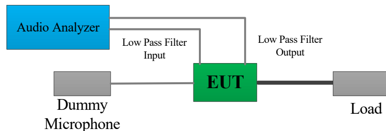
Audio Low Pass Filter Response Test
