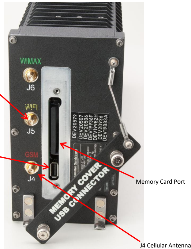
Figure 1: Isometric View of eFAST product on mounting tray (as installed in aircraft)
