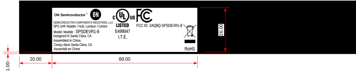
Figure 2 - Label Location on Rear of Enclosure
