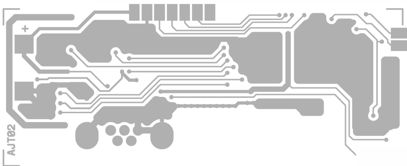
Bottom View - PCB Component Layout - AJT02
