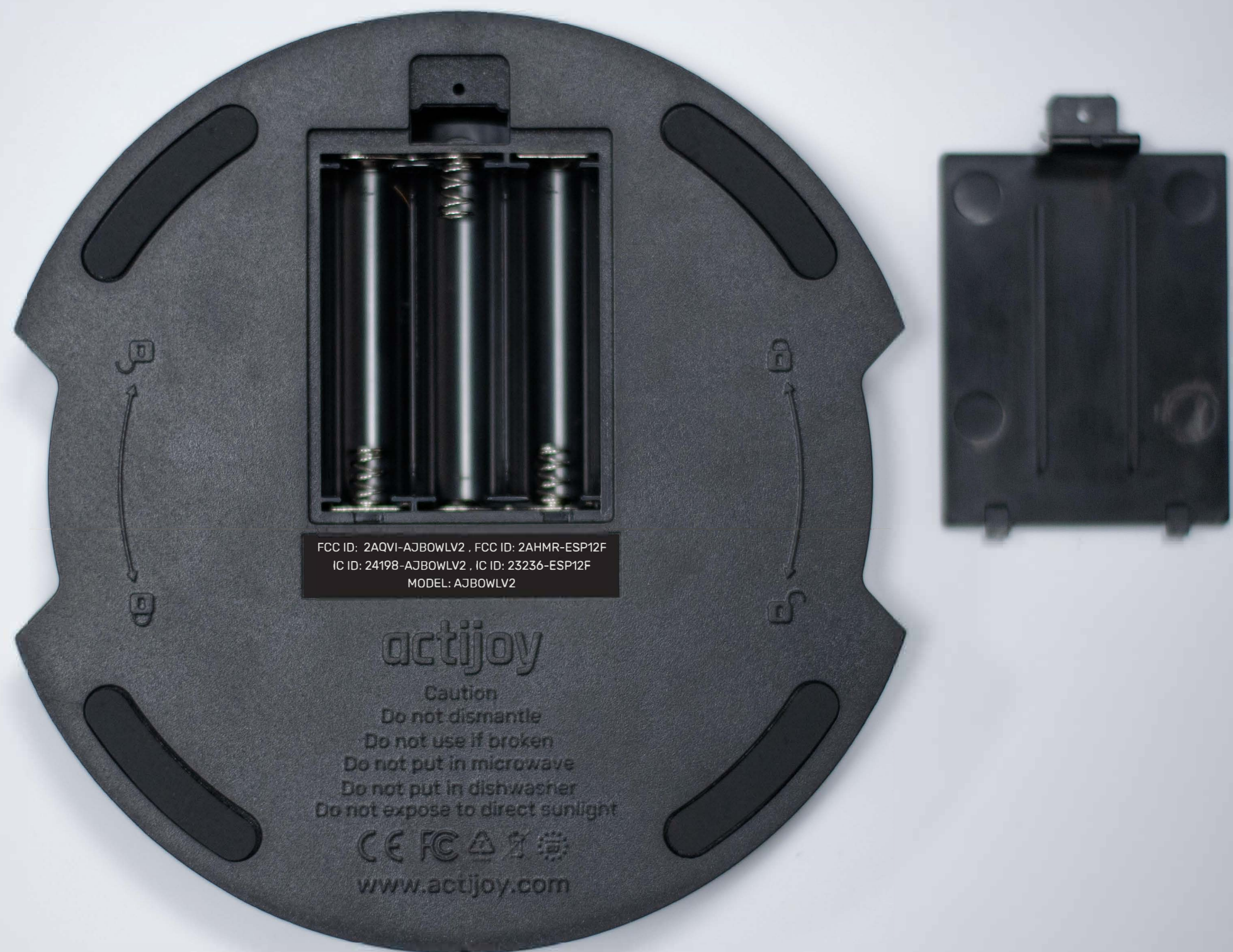
AJBowlV2 - Bottom with Battery Cover Removed
