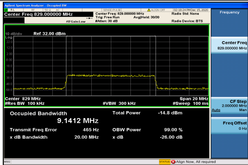
Band5-10MHz-QPSK-20450-50RB#0-9.1412
