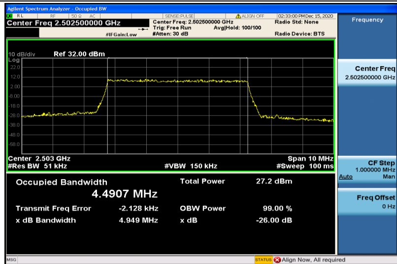
Band7-5MHz-QPSK-20775-25RB#0-4.4907
