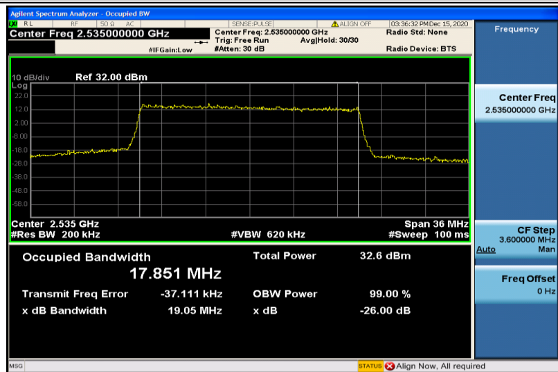
Band7-20MHz-QPSK-21100-100RB#0-17.851
