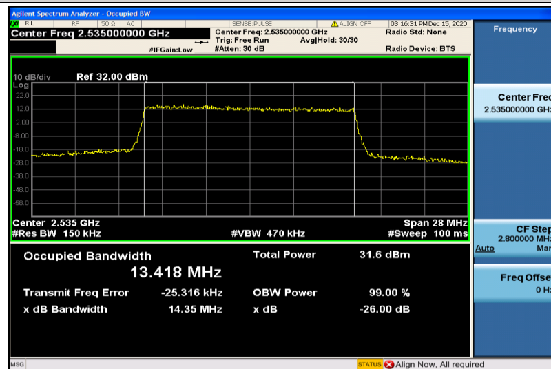
Band7-15MHz-QPSK-21100-75RB#0-13.418
