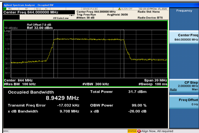
Band5-10MHz-QPSK-20600-50RB#0-8.9429
