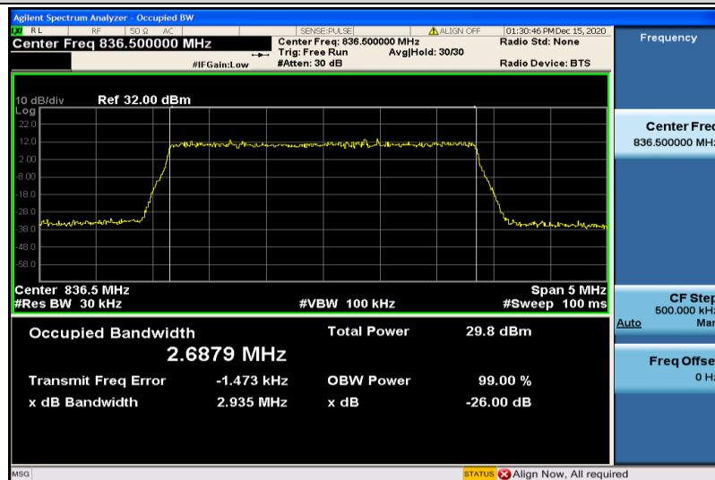
Band5-3MHz-16QAM-20525-15RB#0-2.6879
