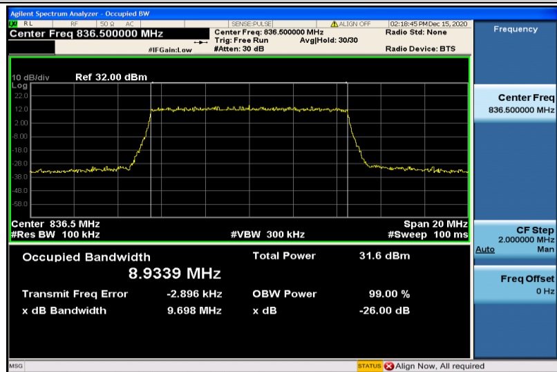
Band5-10MHz-QPSK-20525-50RB#0-8.9339
