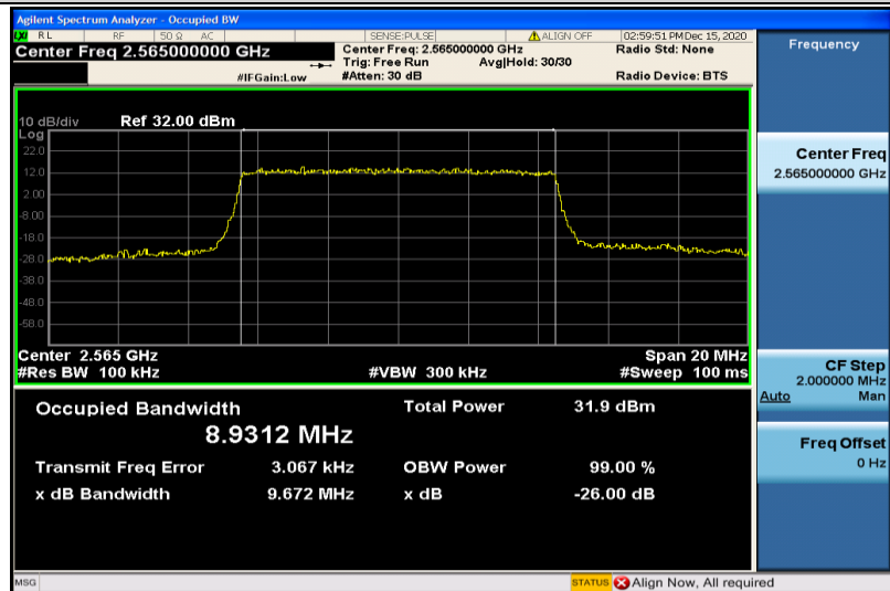
Band7-10MHz-16QAM-21400-50RB#0-8.9312
