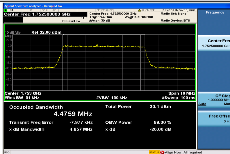
Band4-5MHz-16QAM-20375-25RB#0-4.4759
