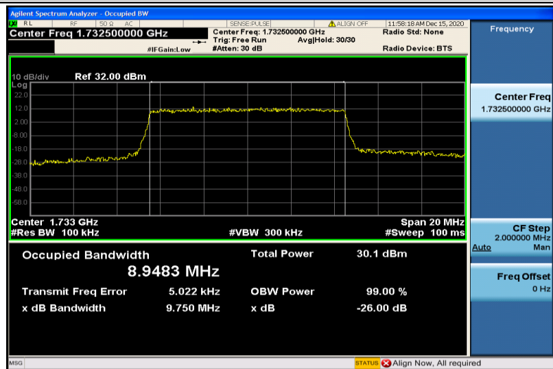
Band4-10MHz-16QAM-20175-50RB#0-8.9483
