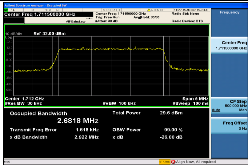
Band4-3MHz-16QAM-19965-15RB#0-2.6818
