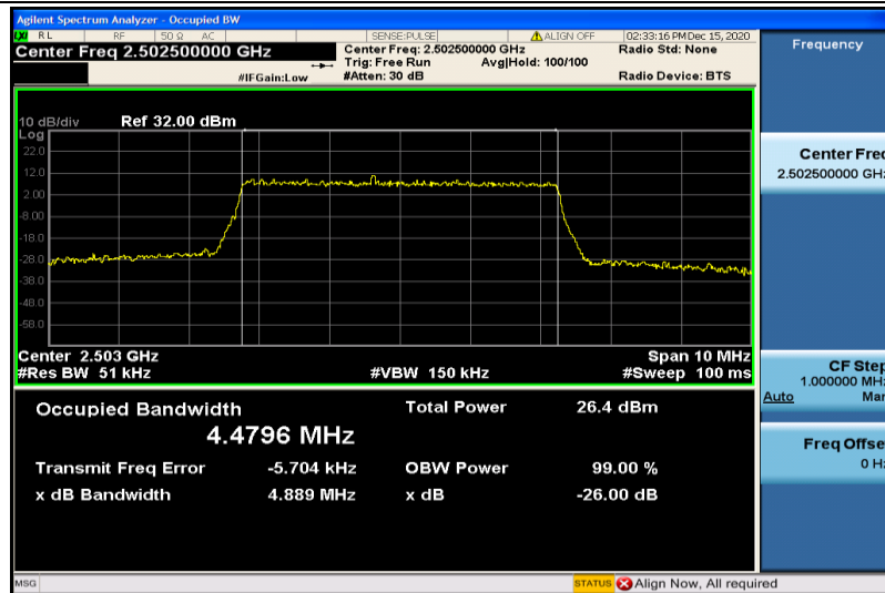
Band7-5MHz-16QAM-20775-25RB#0-4.4796
