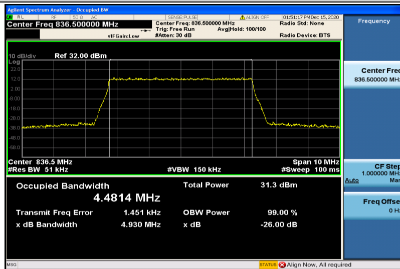
Band5-5MHz-QPSK-20525-25RB#0-4.4814
