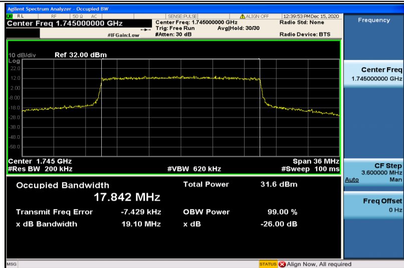
Band4-20MHz-QPSK-20300-100RB#0-17.842
