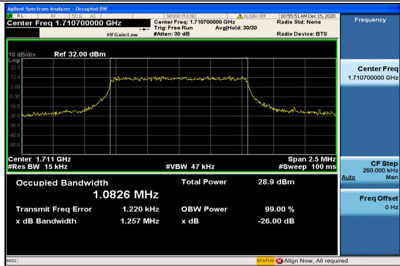
Band4-1.4MHz-16QAM-19957-6RB#0-1.0826
