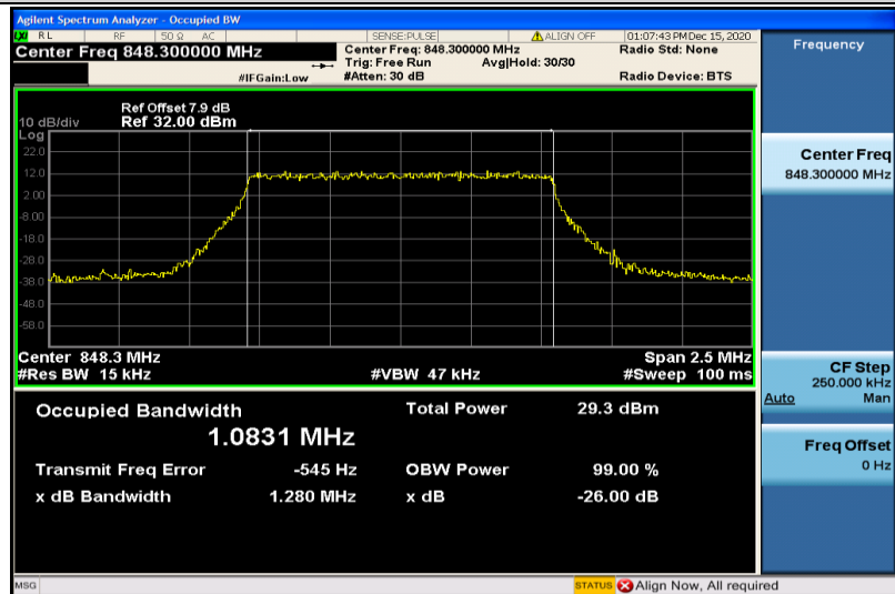
Band5-1.4MHz-16QAM-20643-6RB#0-1.0831
