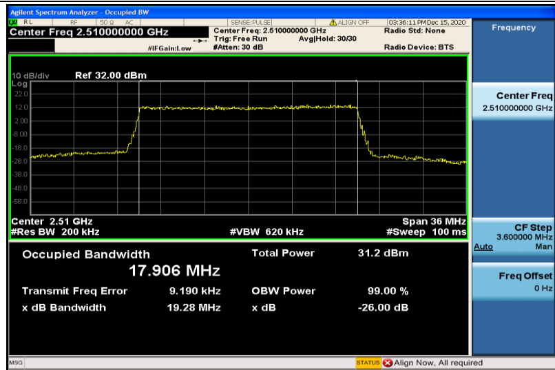
Band7-20MHz-QPSK-20850-100RB#0-17.906
