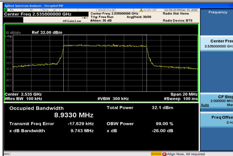
Band7-10MHz-QPSK-21100-50RB#0-8.9330
