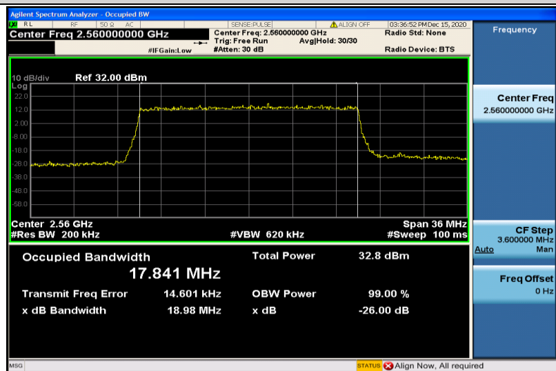
Band7-20MHz-QPSK-21350-100RB#0-17.841
