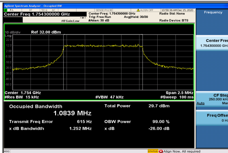
Band4-1.4MHz-QPSK-20393-6RB#0-1.0839
