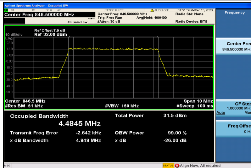
Band5-5MHz-QPSK-20625-25RB#0-4.4845
