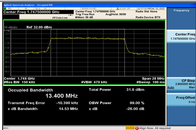
Band4-15MHz-QPSK-20325-75RB#0-13.400
