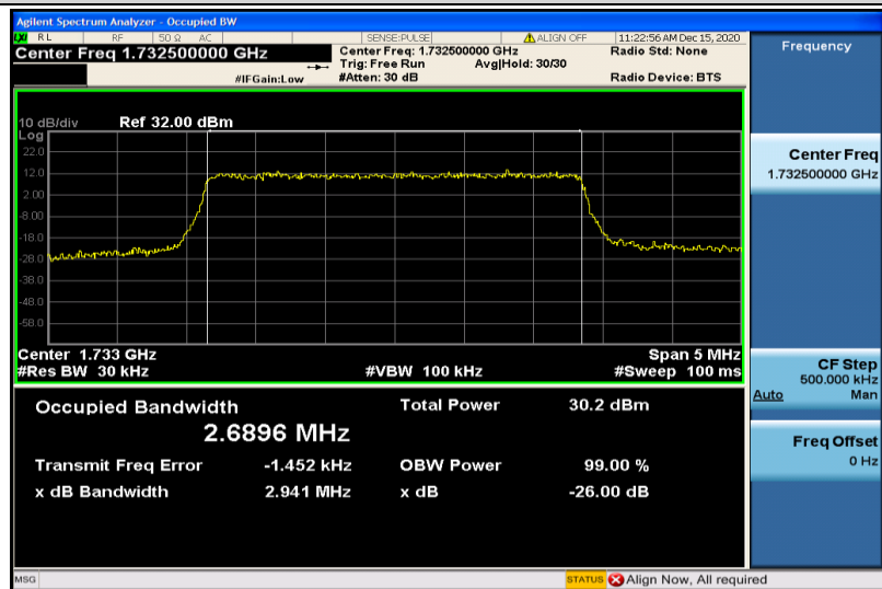
Band4-3MHz-QPSK-20175-15RB#0-2.6896
