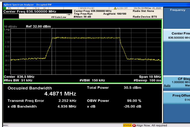
Band5-5MHz-16QAM-20525-25RB#0-4.4871
