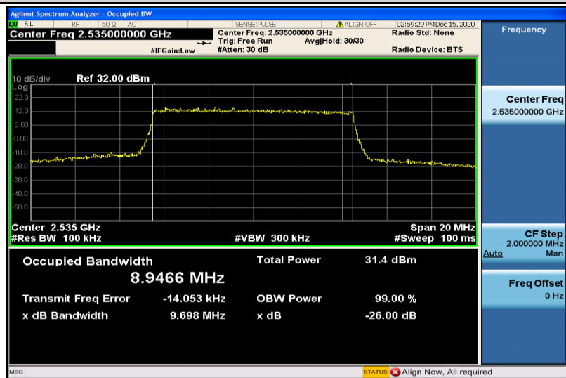
Band7-10MHz-16QAM-21100-50RB#0-8.9466
