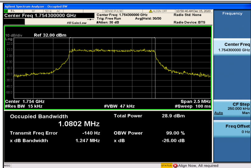
Band4-1.4MHz-16QAM-20393-6RB#0-1.0802
