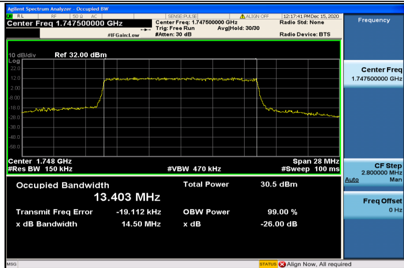
Band4-15MHz-16QAM-20325-75RB#0-13.403
