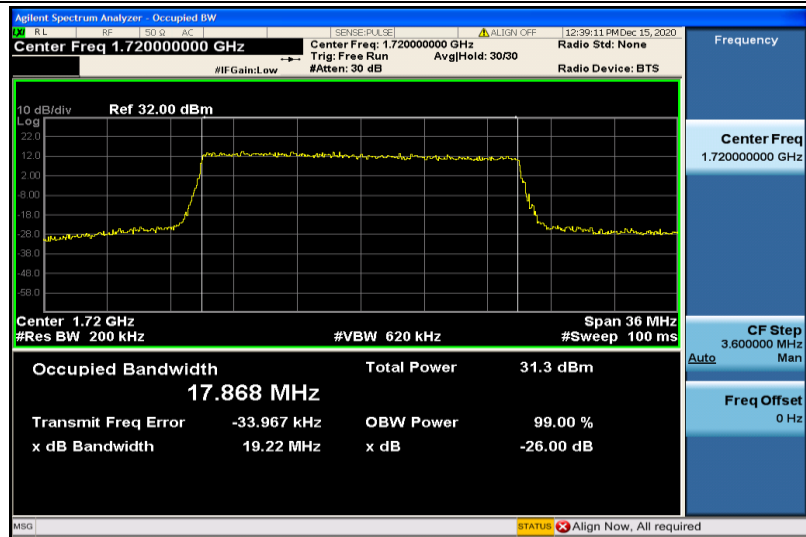
Band4-20MHz-QPSK-20050-100RB#0-17.868
