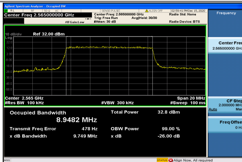
Band7-10MHz-QPSK-21400-50RB#0-8.9482
