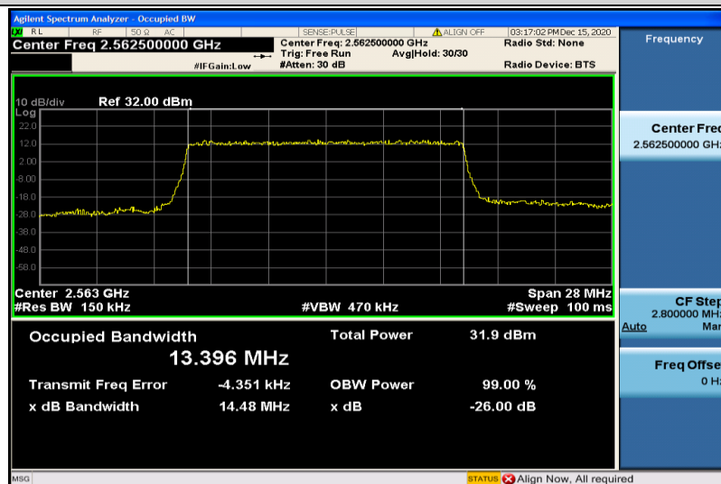
Band7-15MHz-16QAM-21375-75RB#0-13.396
