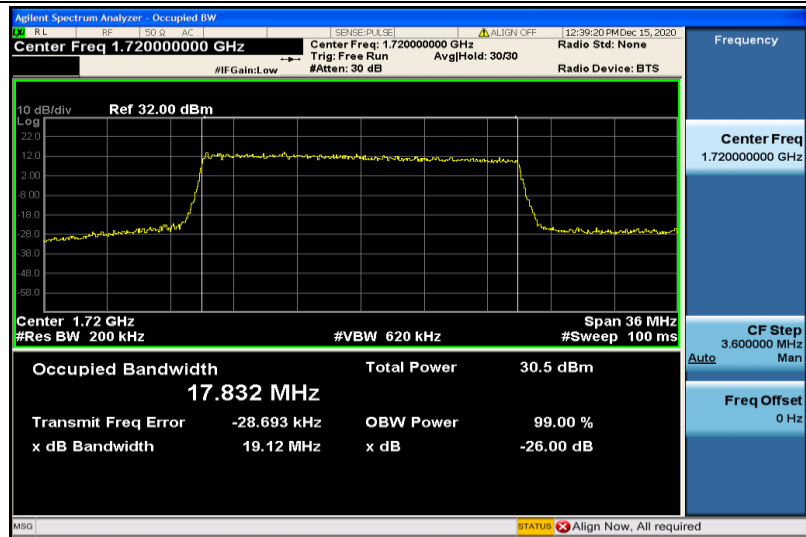
Band4-20MHz-16QAM-20050-100RB#0-17.832
