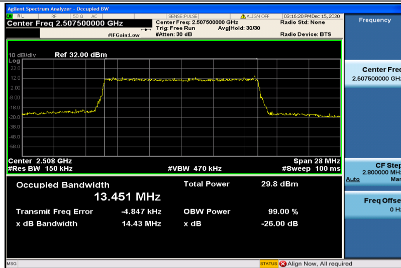
Band7-15MHz-16QAM-20825-75RB#0-13.451
