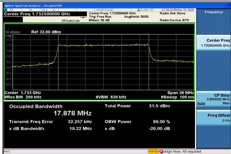
Band4-20MHz-QPSK-20175-100RB#0-17.878
