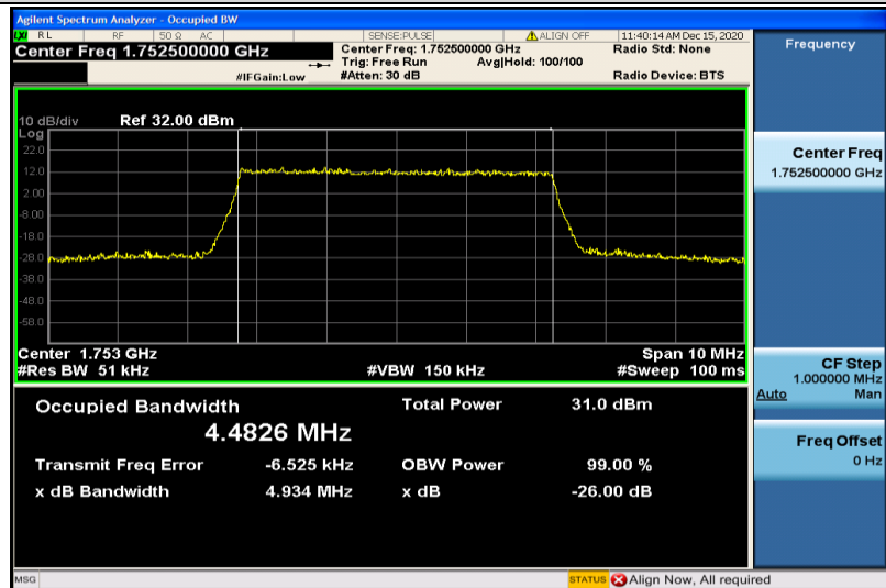
Band4-5MHz-QPSK-20375-25RB#0-4.4826
