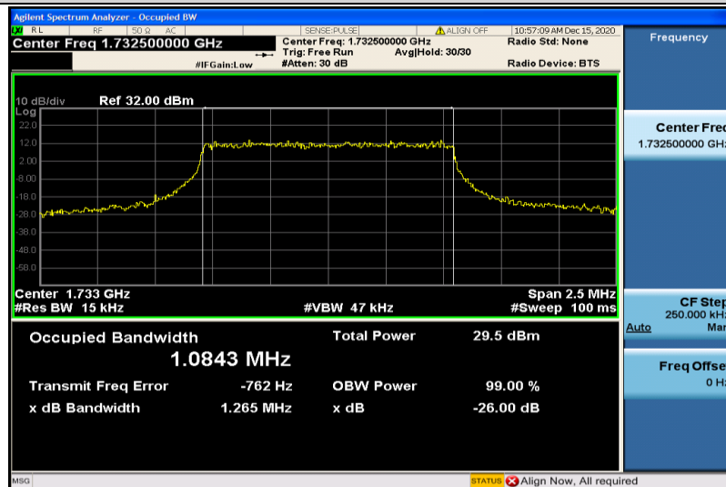
Band4-1.4MHz-QPSK-20175-6RB#0-1.0843
