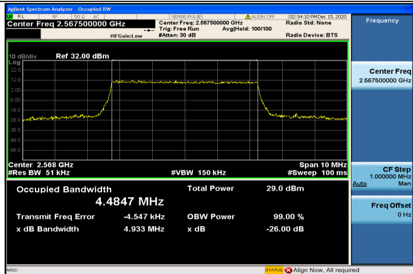
Band7-5MHz-QPSK-21425-25RB#0-4.4847
