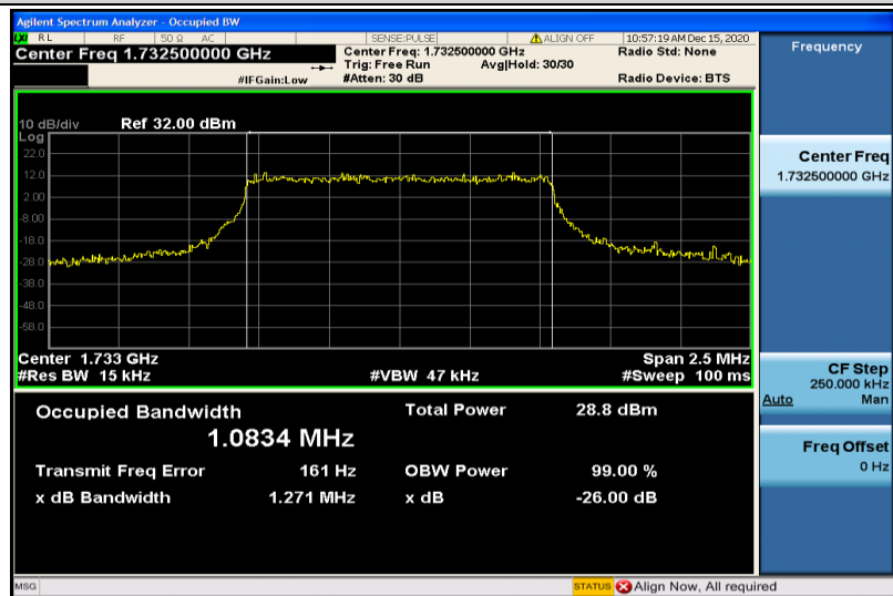
Band4-1.4MHz-16QAM-20175-6RB#0-1.0834
