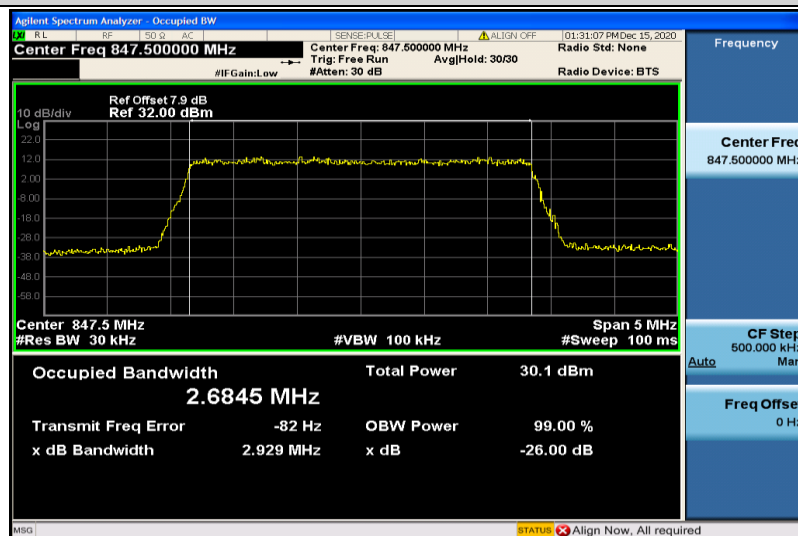
Band5-3MHz-16QAM-20635-15RB#0-2.6845
