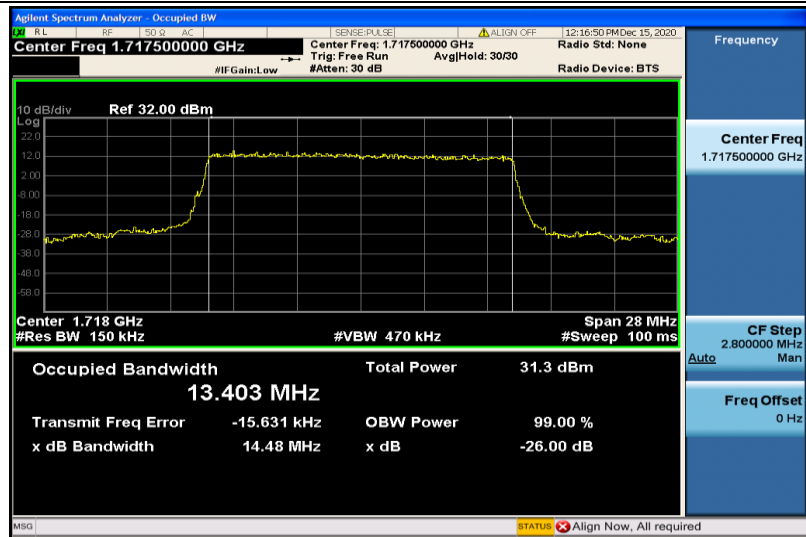
Band4-15MHz-QPSK-20025-75RB#0-13.403
