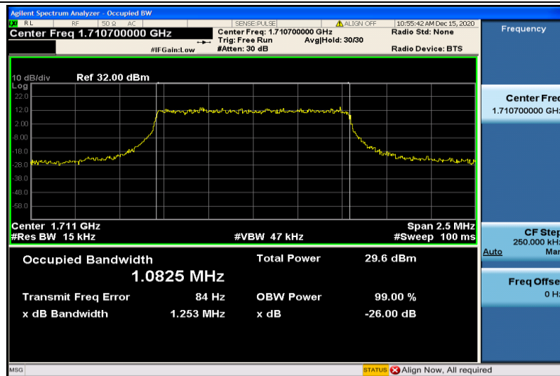
Band4-1.4MHz-QPSK-19957-6RB#0-1.0825
