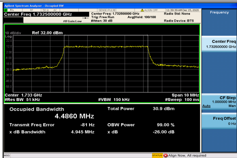
Band4-5MHz-QPSK-20175-25RB#0-4.4860
