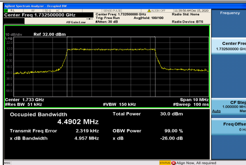
Band4-5MHz-16QAM-20175-25RB#0-4.4902
