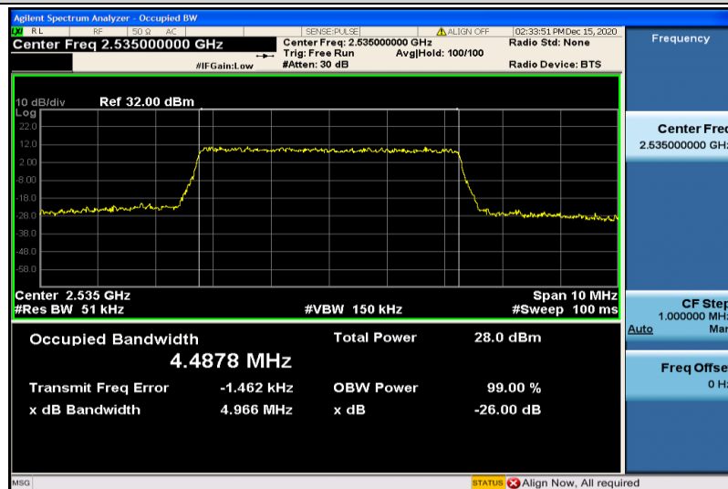
Band7-5MHz-16QAM-21100-25RB#0-4.4878
