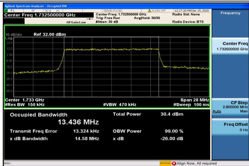
Band4-15MHz-16QAM-20175-75RB#0-13.436
