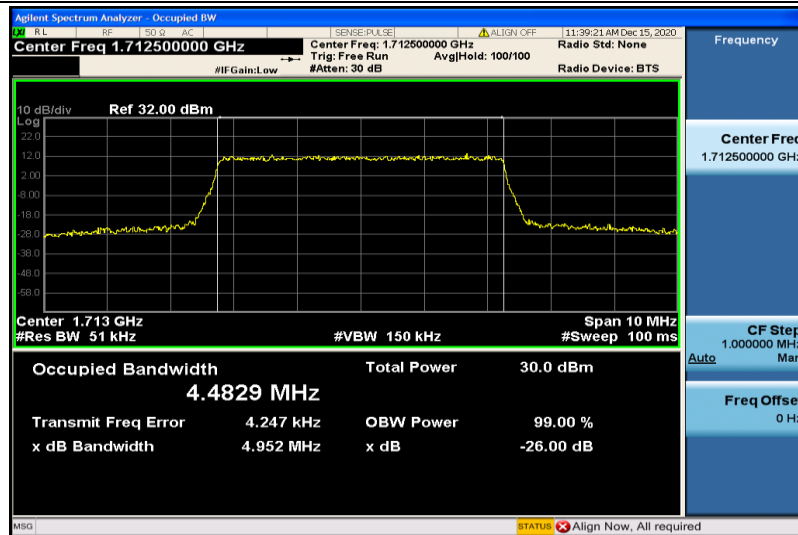
Band4-5MHz-16QAM-19975-25RB#0-4.4829
