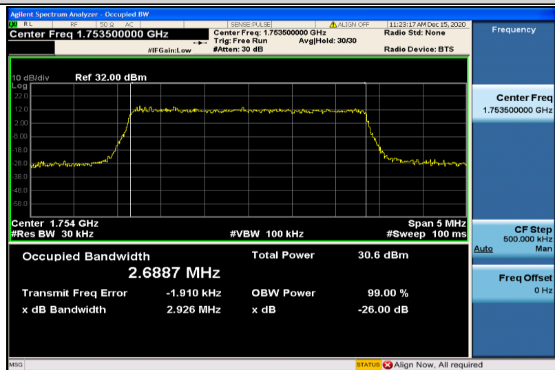
Band4-3MHz-QPSK-20385-15RB#0-2.6887
