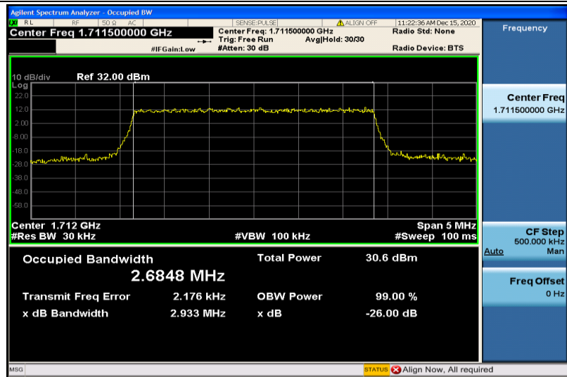
Band4-3MHz-QPSK-19965-15RB#0-2.6848
