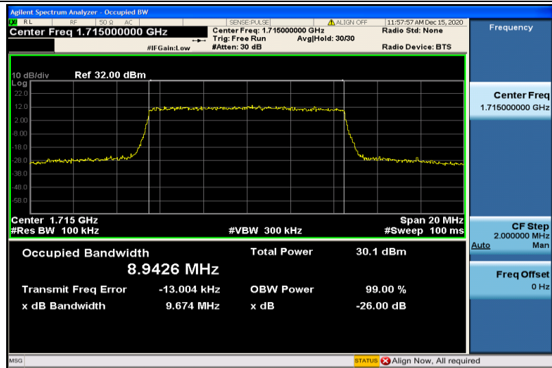
Band4-10MHz-16QAM-20000-50RB#0-8.9426
