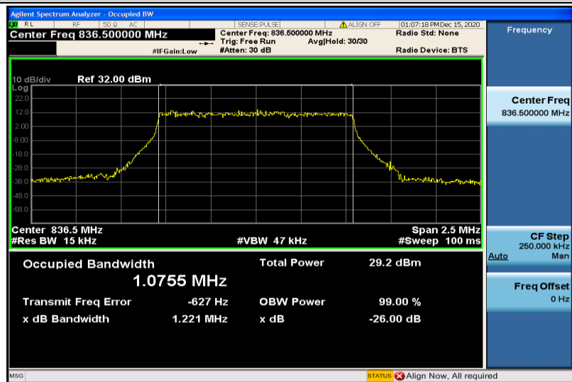
Band5-1.4MHz-16QAM-20525-6RB#0-1.0755
