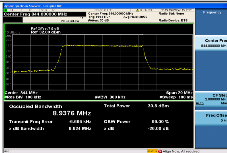
Band5-10MHz-16QAM-20600-50RB#0-8.9376
