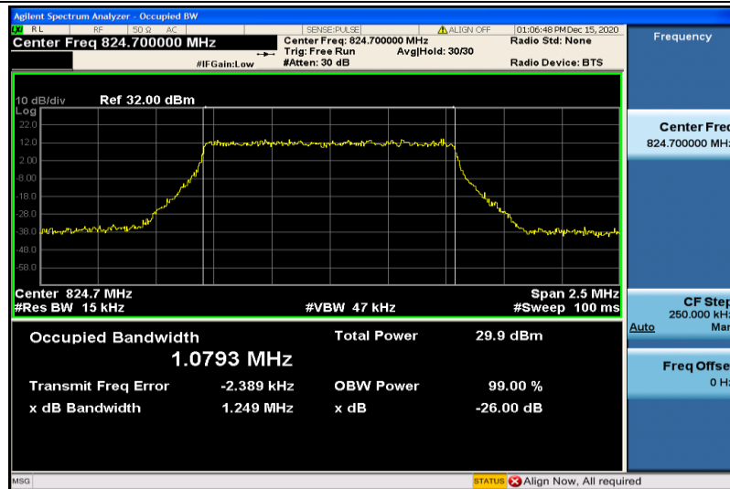
Band5-1.4MHz-QPSK-20407-6RB#0-1.0793
