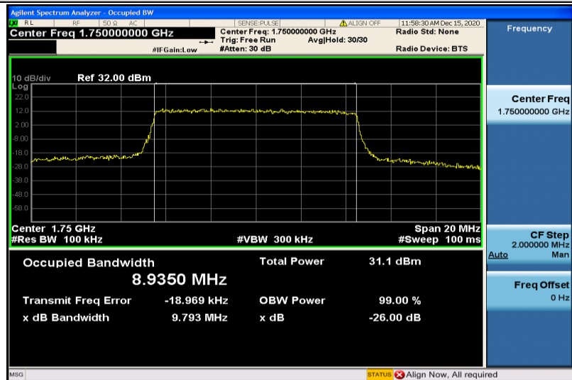
Band4-10MHz-QPSK-20350-50RB#0-8.9350
