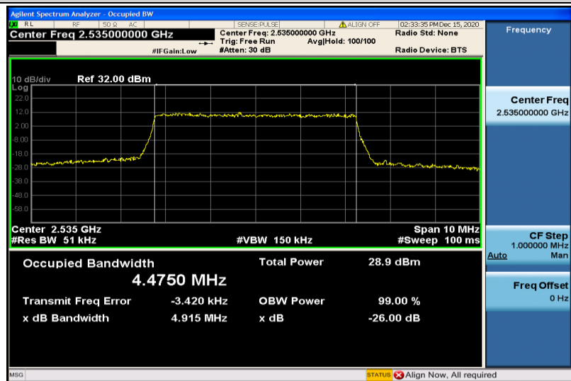
Band7-5MHz-QPSK-21100-25RB#0-4.4750
