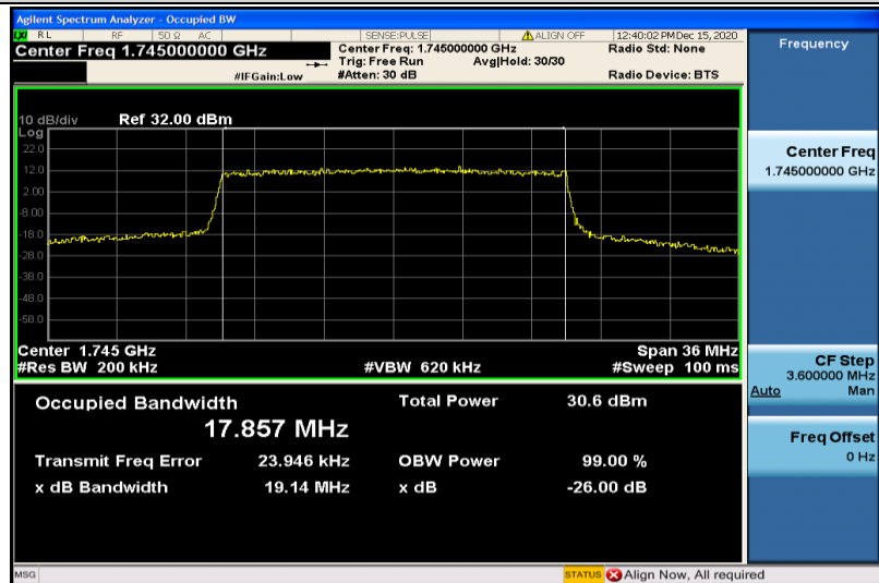
Band4-20MHz-16QAM-20300-100RB#0-17.857
