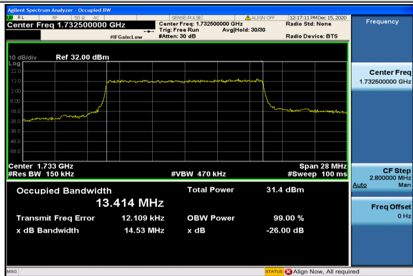
Band4-15MHz-QPSK-20175-75RB#0-13.414
