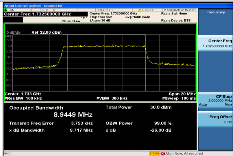
Band4-10MHz-QPSK-20175-50RB#0-8.9449
