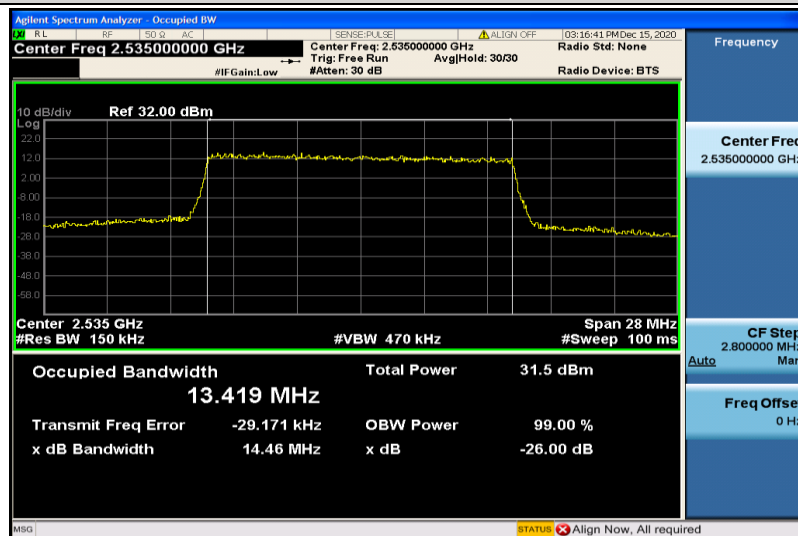
Band7-15MHz-16QAM-21100-75RB#0-13.419
