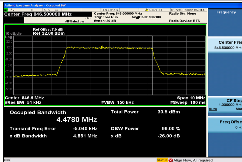
Band5-5MHz-16QAM-20625-25RB#0-4.4780
