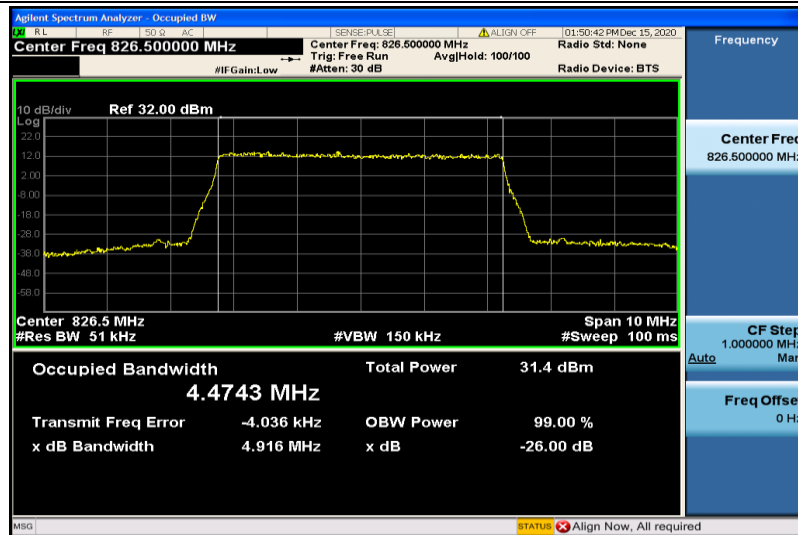
Band5-5MHz-QPSK-20425-25RB#0-4.4743
