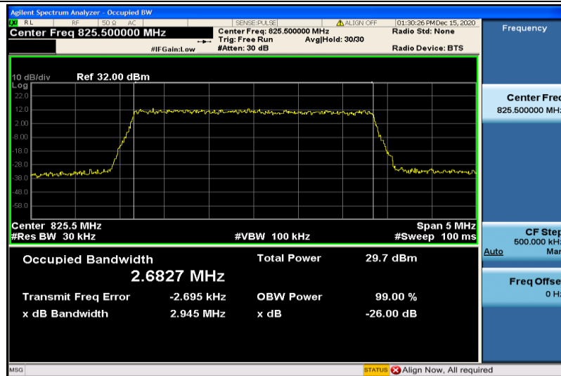
Band5-3MHz-16QAM-20415-15RB#0-2.6827
