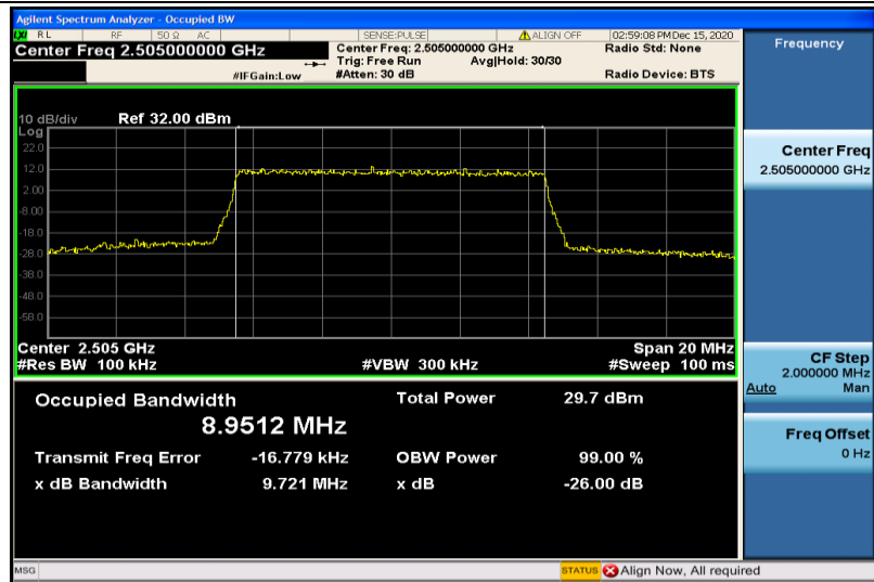
Band7-10MHz-16QAM-20800-50RB#0-8.9512
