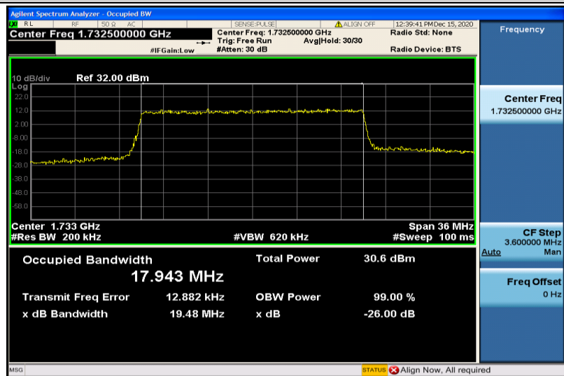
Band4-20MHz-16QAM-20175-100RB#0-17.943
