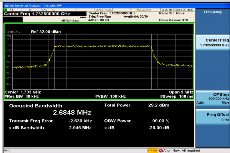
Band4-3MHz-16QAM-20175-15RB#0-2.6848
