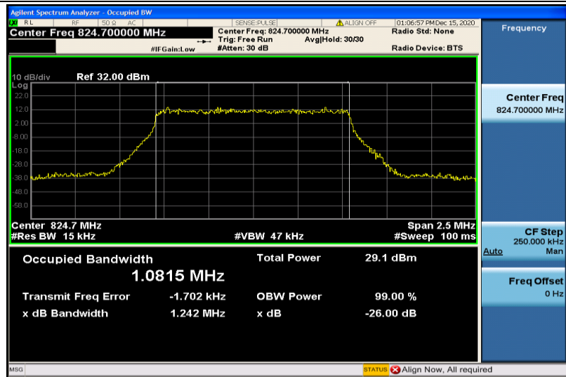
Band5-1.4MHz-16QAM-20407-6RB#0-1.0815
