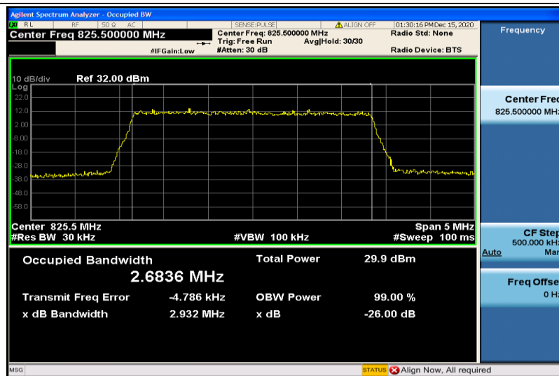
Band5-3MHz-QPSK-20415-15RB#0-2.6836
