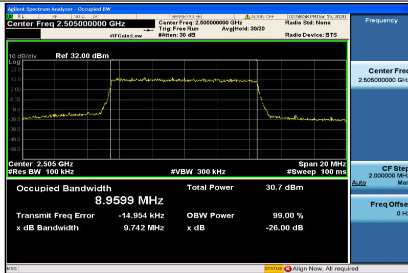
Band7-10MHz-QPSK-20800-50RB#0-8.9599
