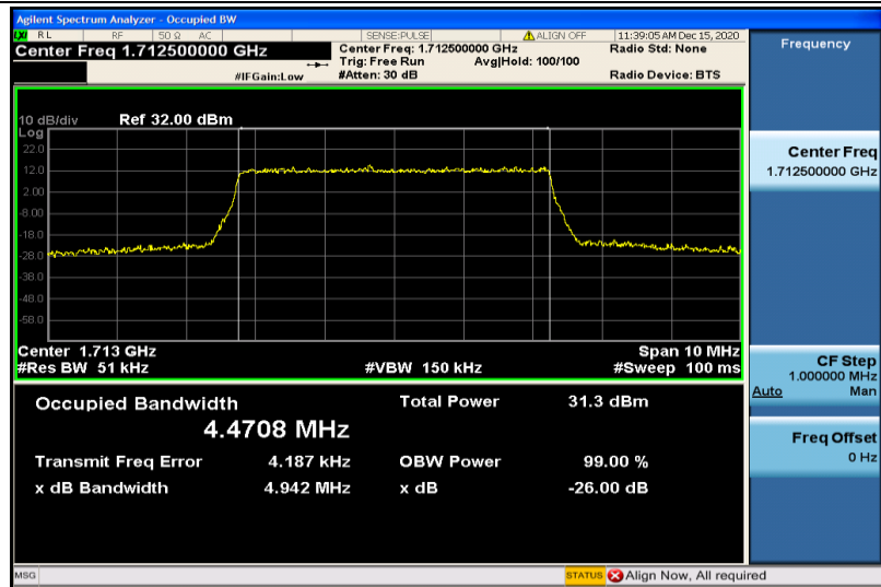
Band4-5MHz-QPSK-19975-25RB#0-4.4708
