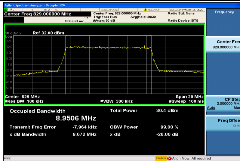
Band5-10MHz-16QAM-20450-50RB#0-8.9506
