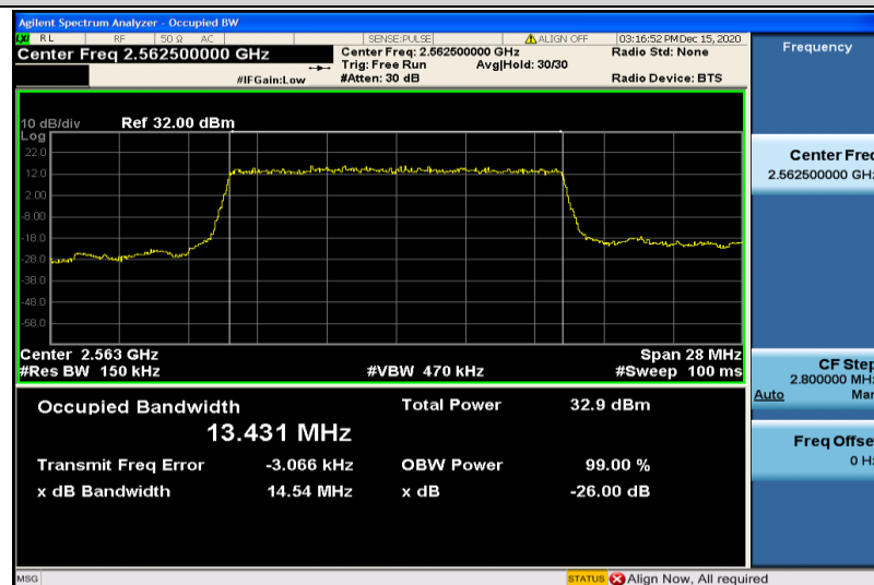
Band7-15MHz-QPSK-21375-75RB#0-13.431
