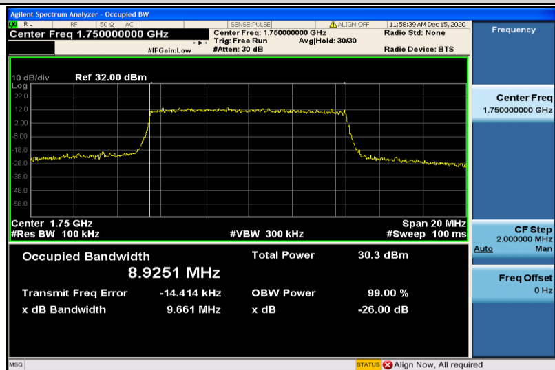
Band4-10MHz-16QAM-20350-50RB#0-8.9251
