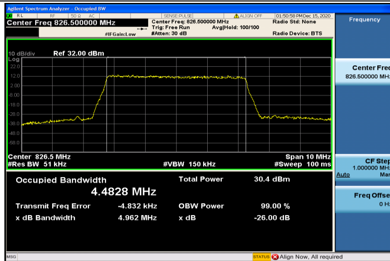
Band5-5MHz-16QAM-20425-25RB#0-4.4828
