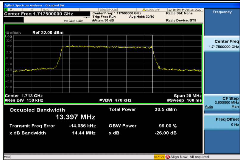
Band4-15MHz-16QAM-20025-75RB#0-13.397
