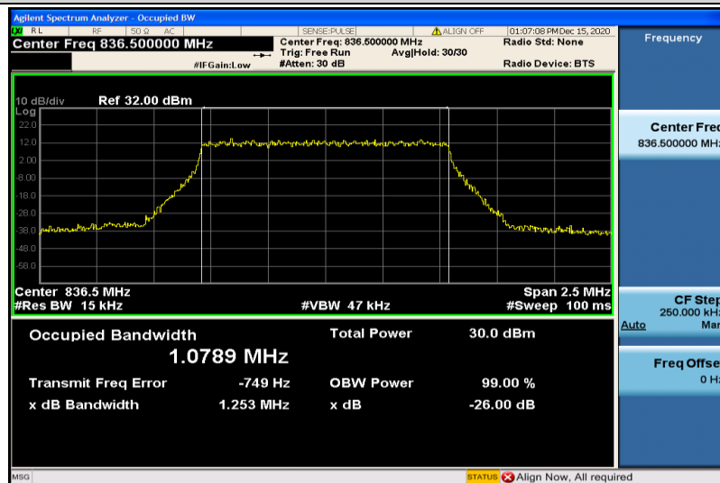
Band5-1.4MHz-QPSK-20525-6RB#0-1.0789
