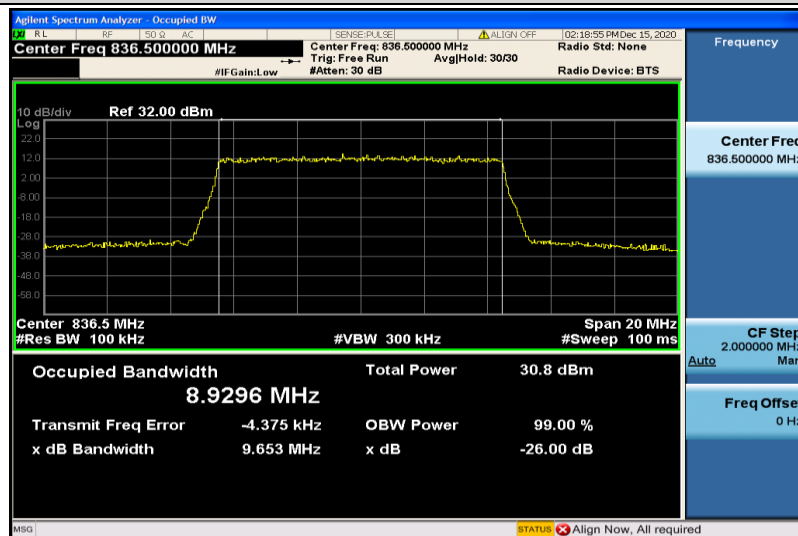
Band5-10MHz-16QAM-20525-50RB#0-8.9296
