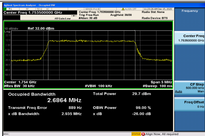
Band4-3MHz-16QAM-20385-15RB#0-2.6864
