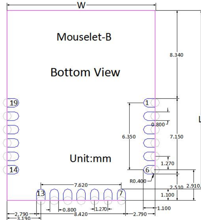
Figure 3: Mechanical Information
