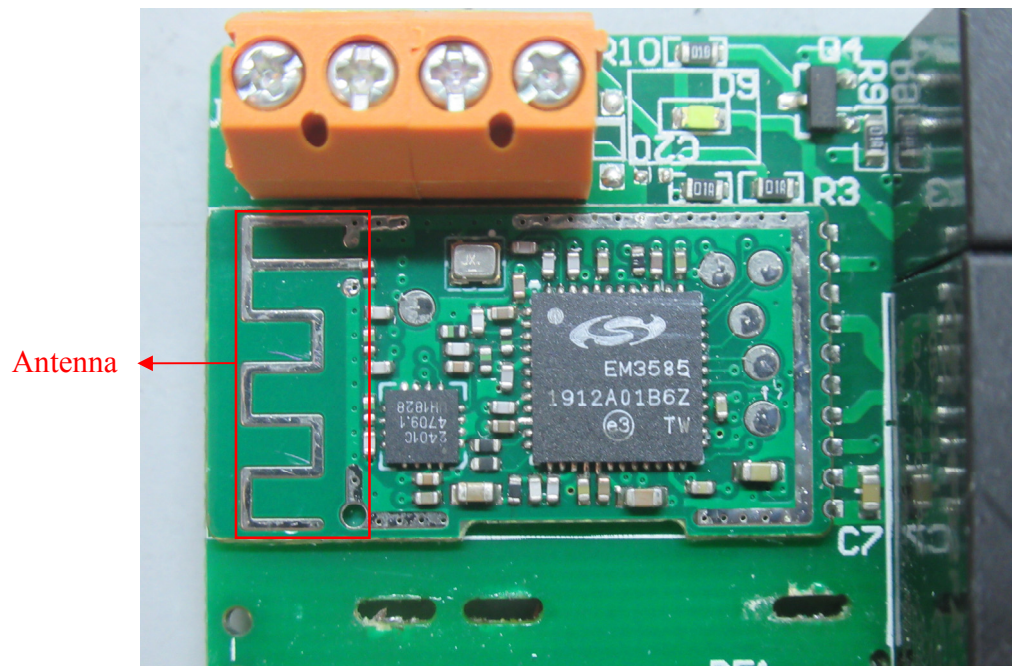
EUT(TERNCY-SM01-D3) – PCB-2 Top Chip View
