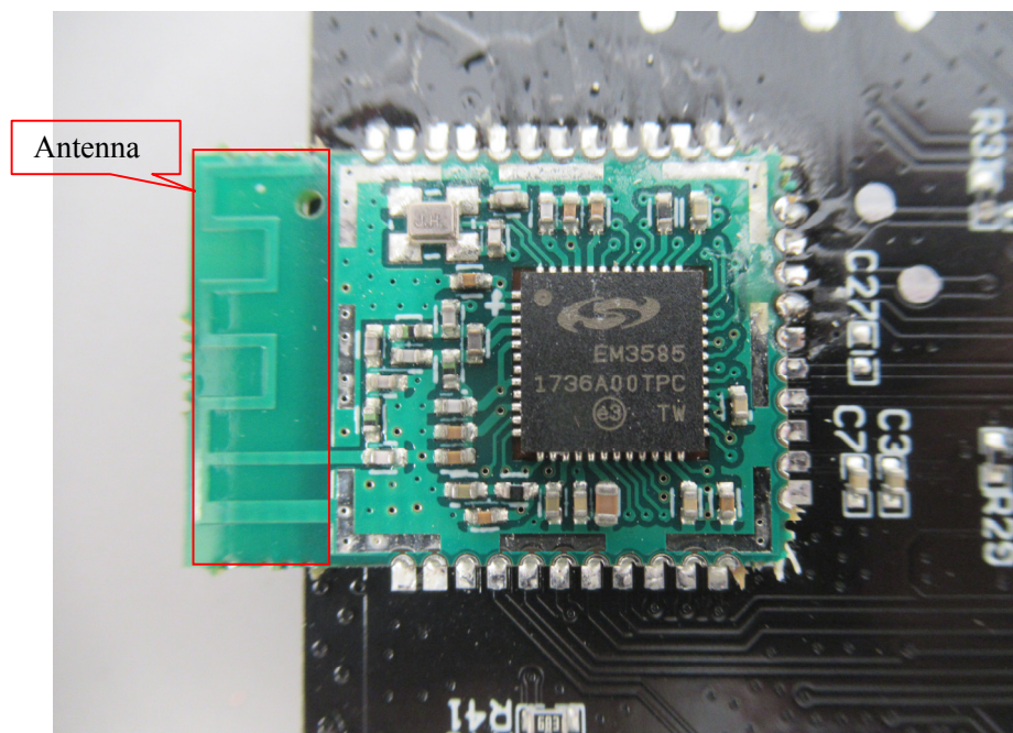
EUT – Module Top View
