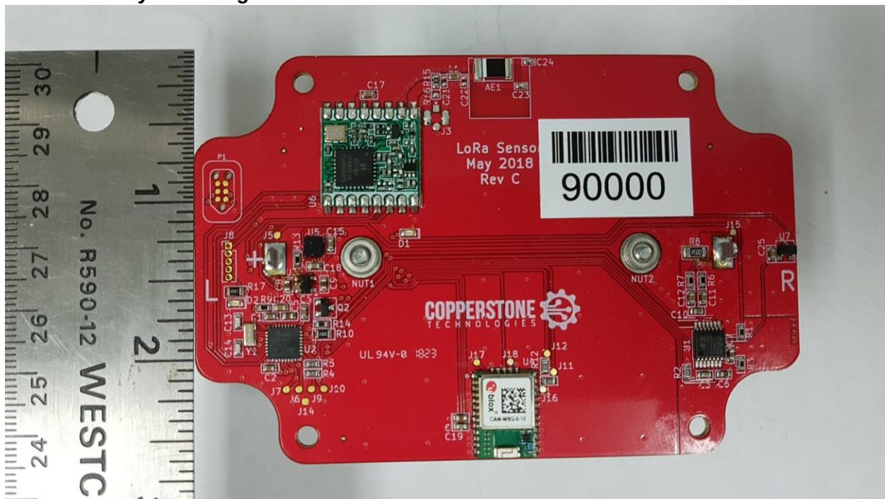
PCB assembly short edge
