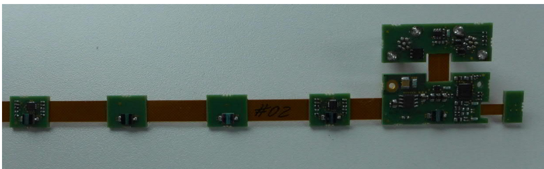
212050_EUT_03c:PCB RFID reader view 3 *1
