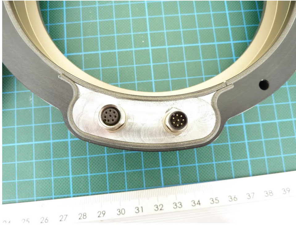
212050_eut_09: EUT connector view
