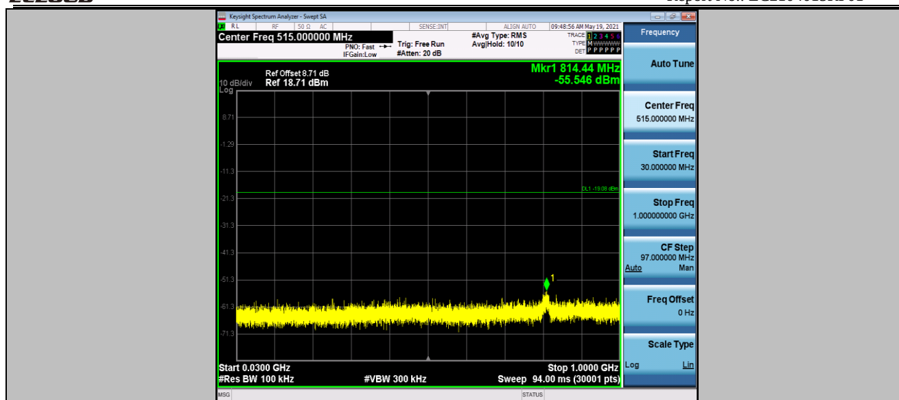
11N20SISO_Ant1_2437_30~1000
