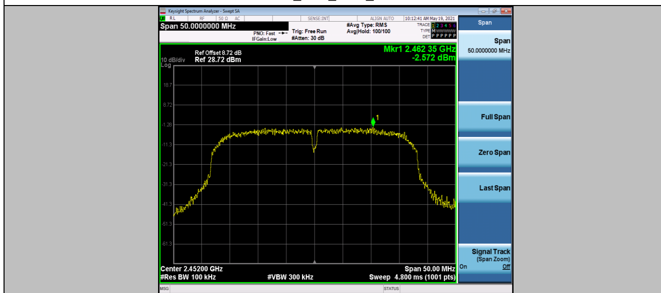
11N40SISO_Ant1_2452_0-Reference
