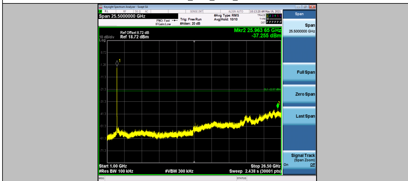
11N40SISO_Ant1_2452_1000~26500
