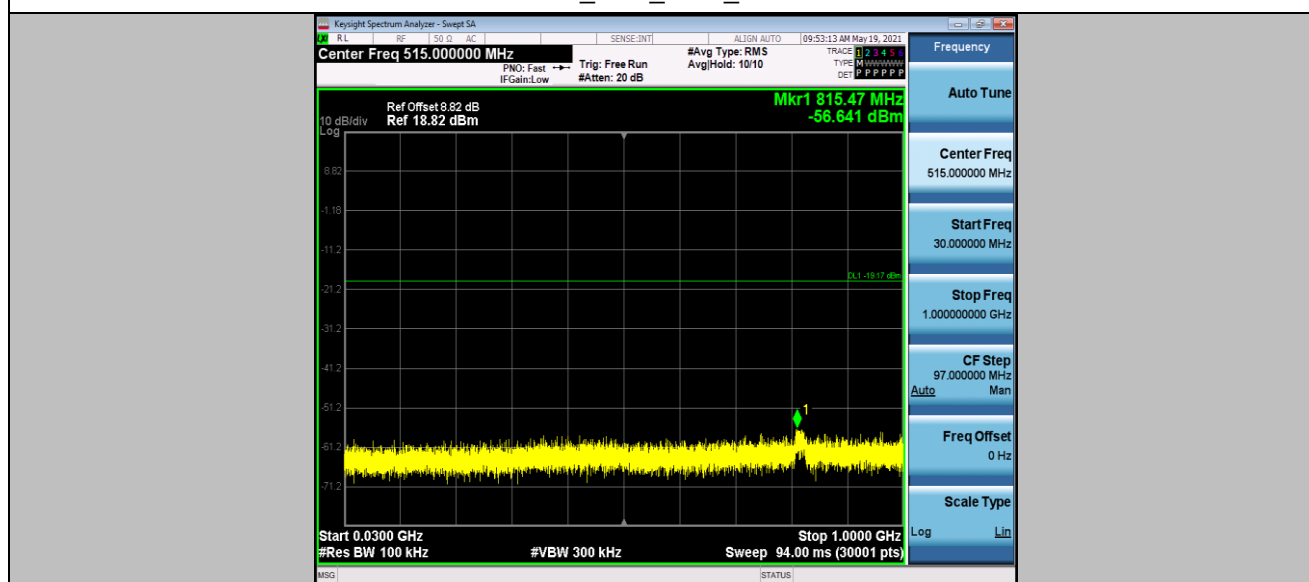
11N20SISO_Ant1_2462_30-1000
