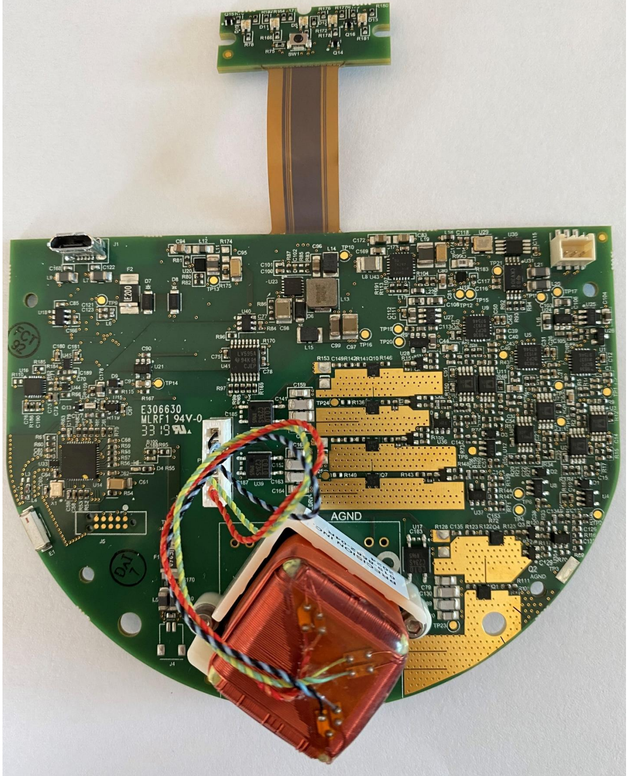
PCBA Front
