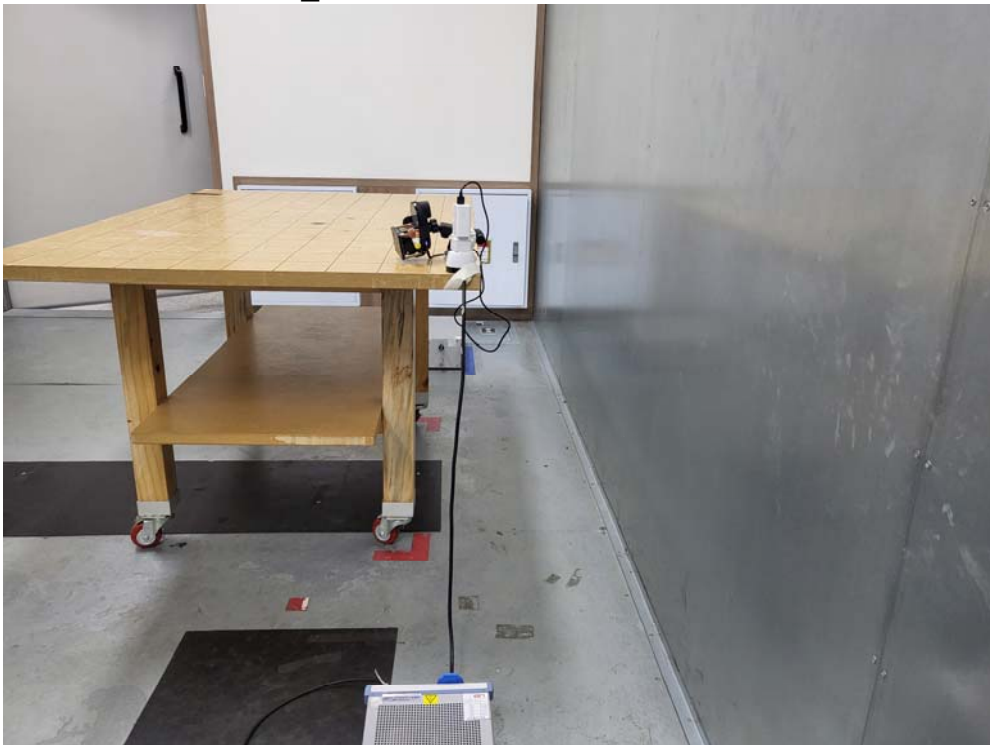
Conducted Emission_Rear
