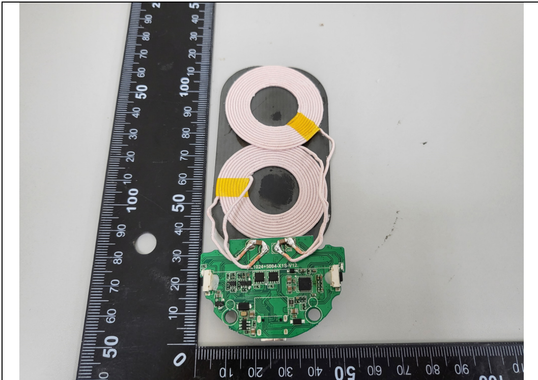
Main Board + Coil Antenna Front
