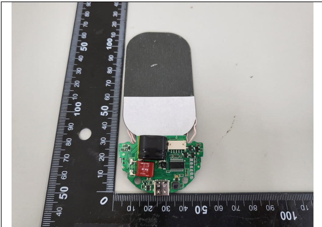
Main Board + Coil Antenna Rear
